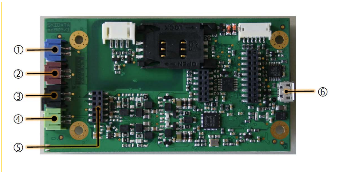
Fig. 5: Connectors sd905
