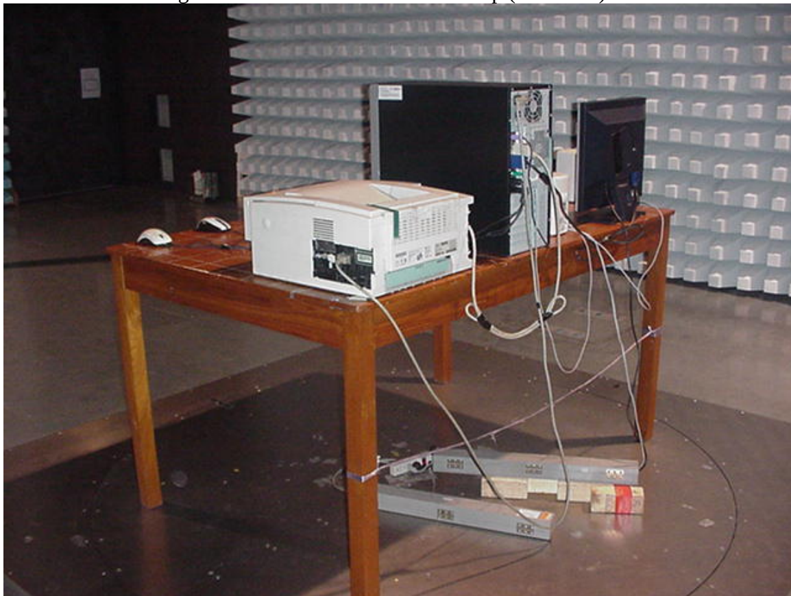
Figure 4-Radiated emission Test set up (rear view)
