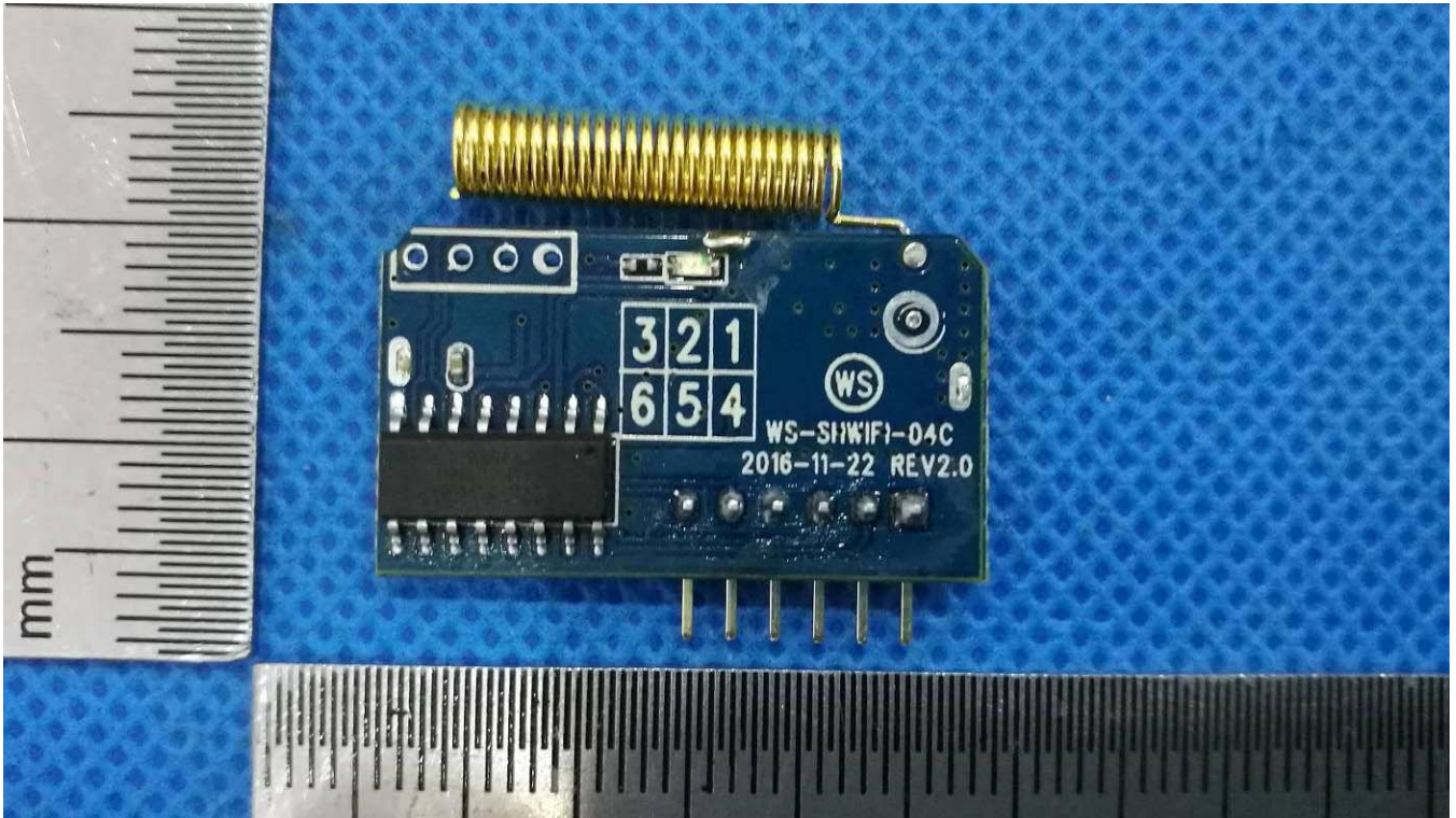
Testing Adapter Board (PCBA)
