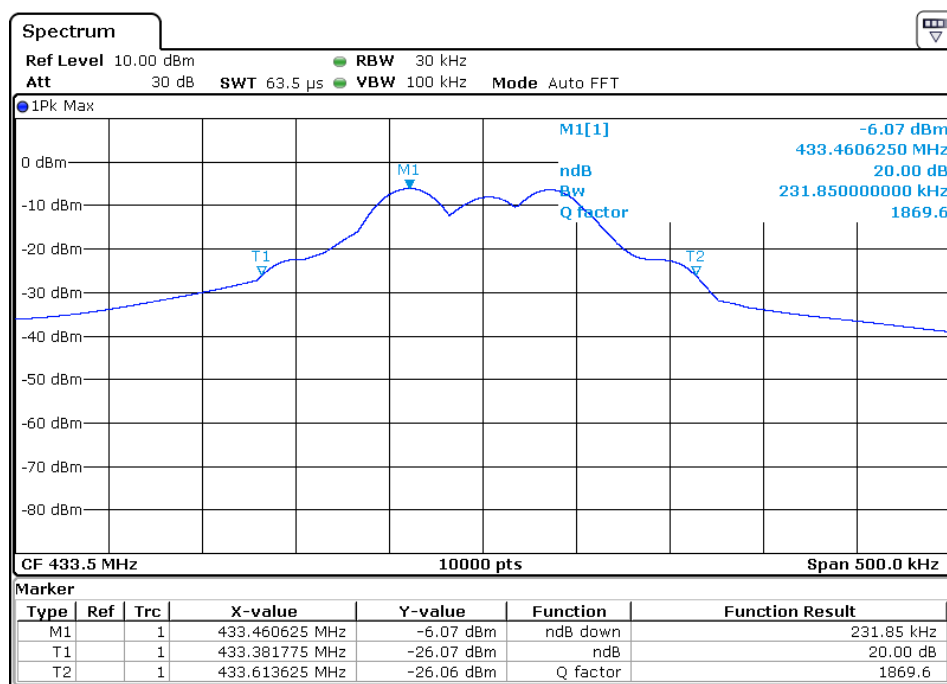
Channel 01: 433.50MHz
