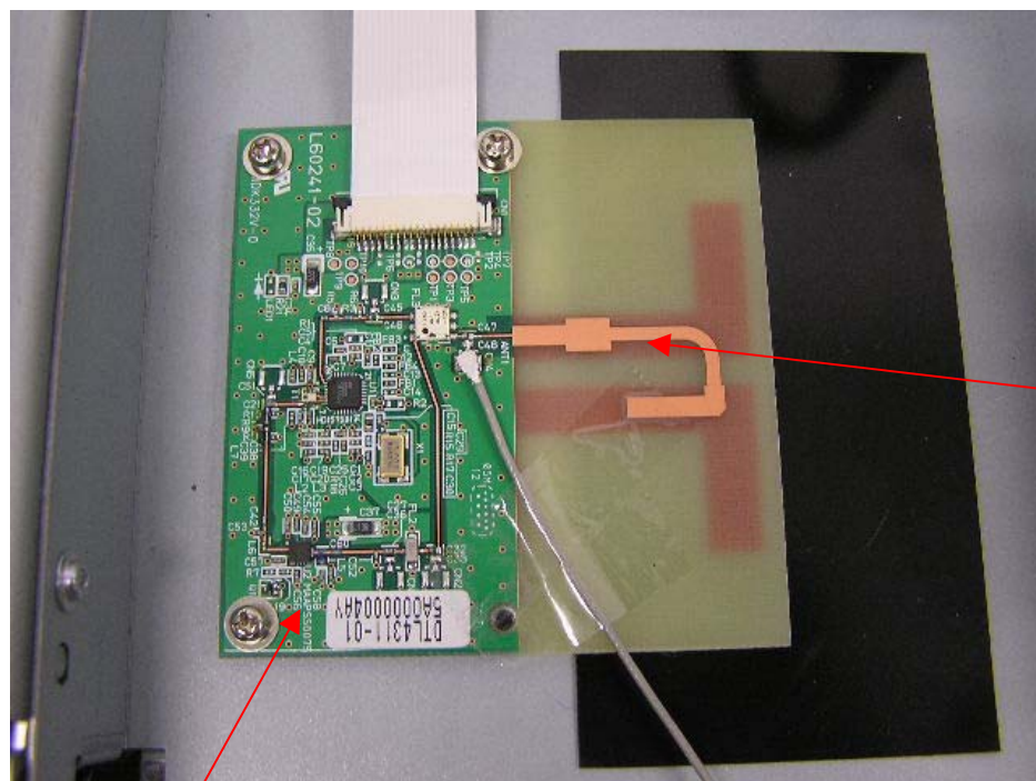
RF PWB Location2
