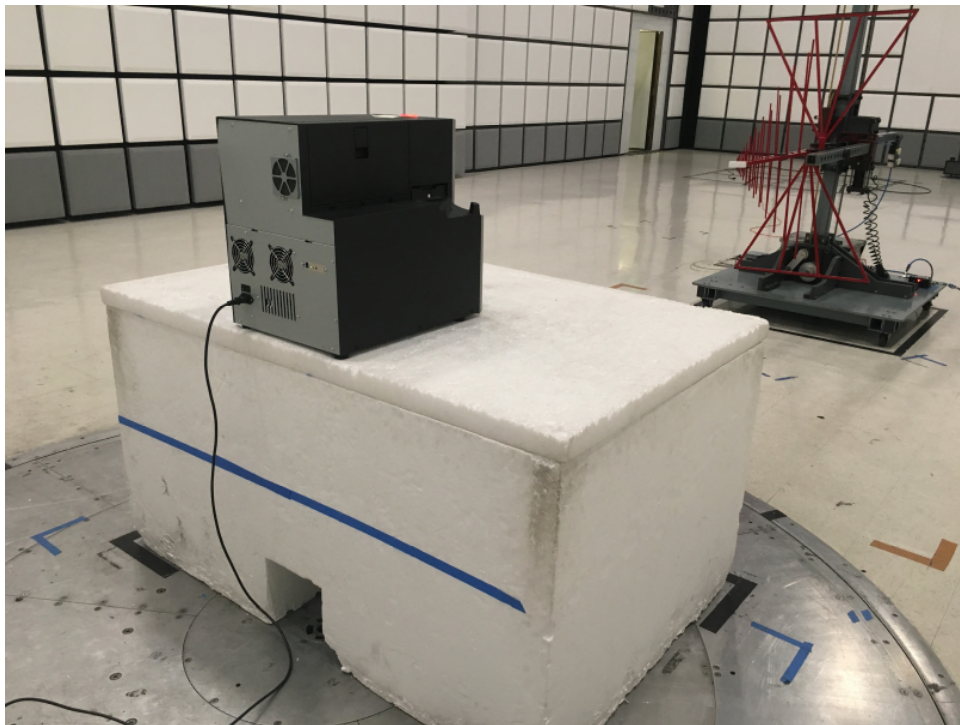
Radiated Spurious Emissions Below 1GHz Rear
