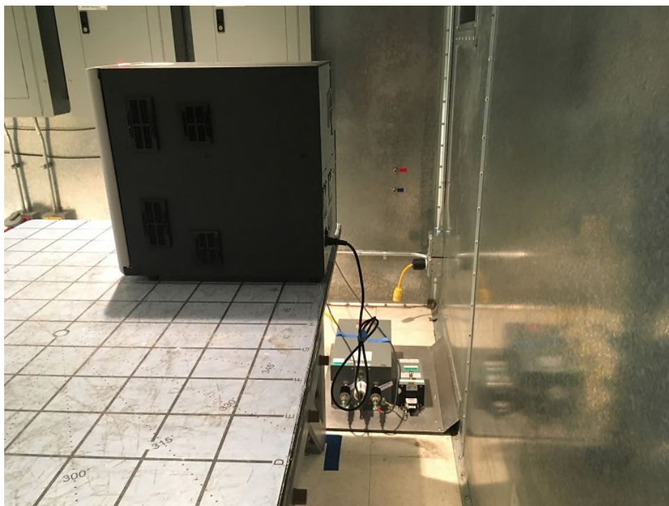
Conducted Emissions Testing
