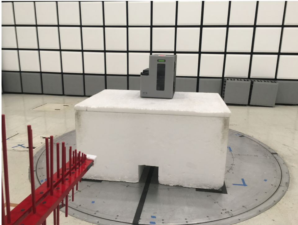
Radiated Spurious Emissions Below 1GHz Front
