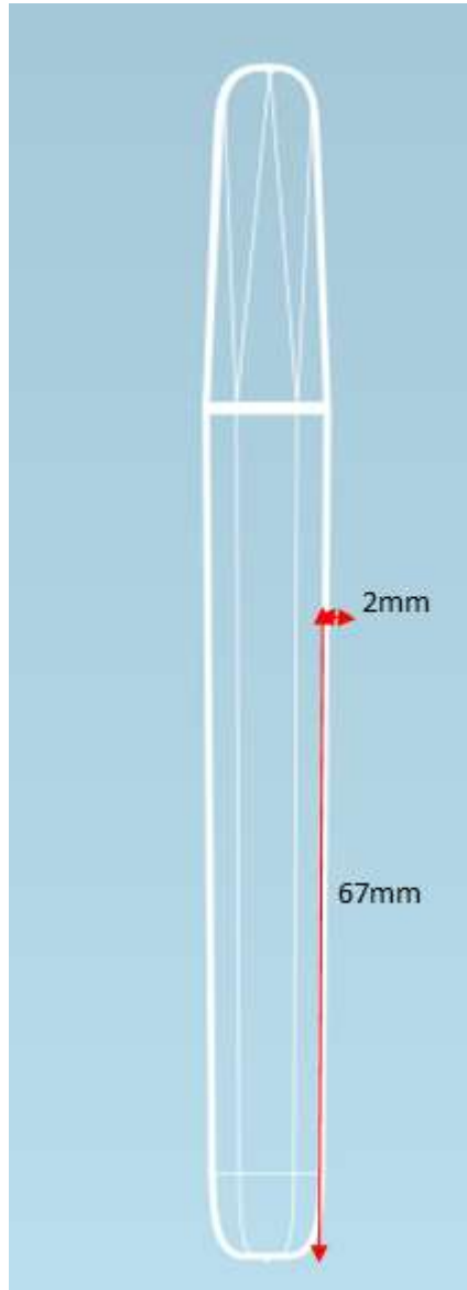
Fig.14.1 EUT Antenna Locations
