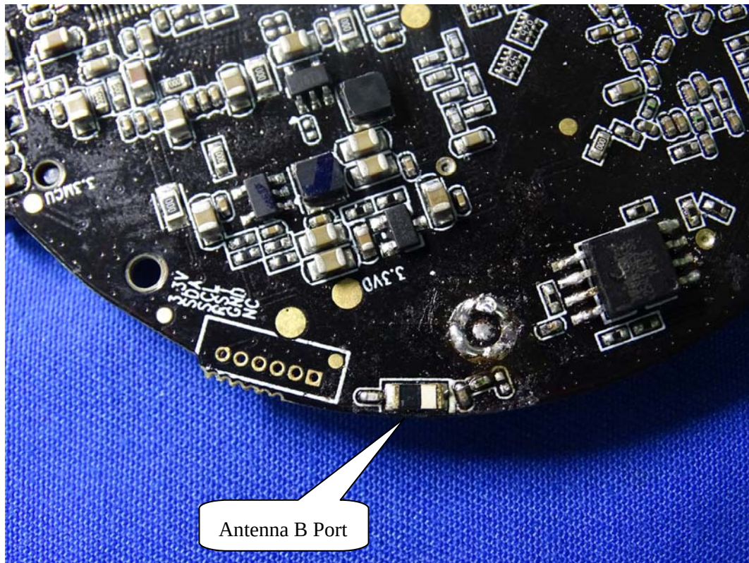
(17) EUT Photo-2.4G Antenna
