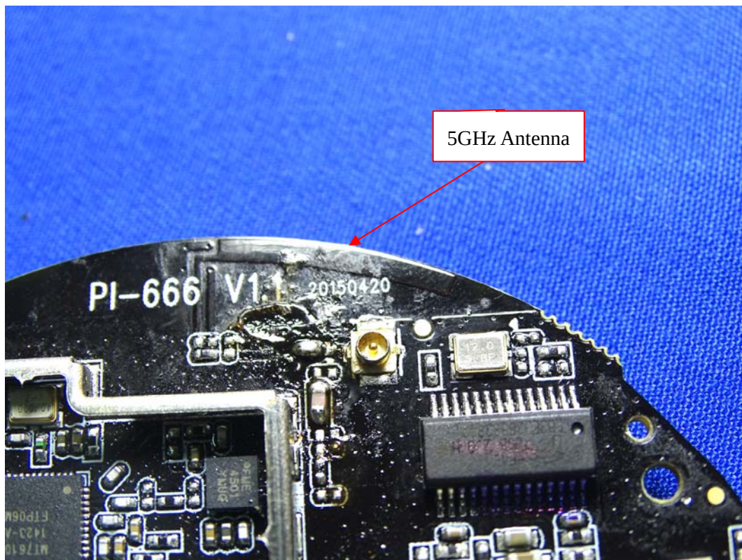
(27) EUT Photo-5G Antenna
