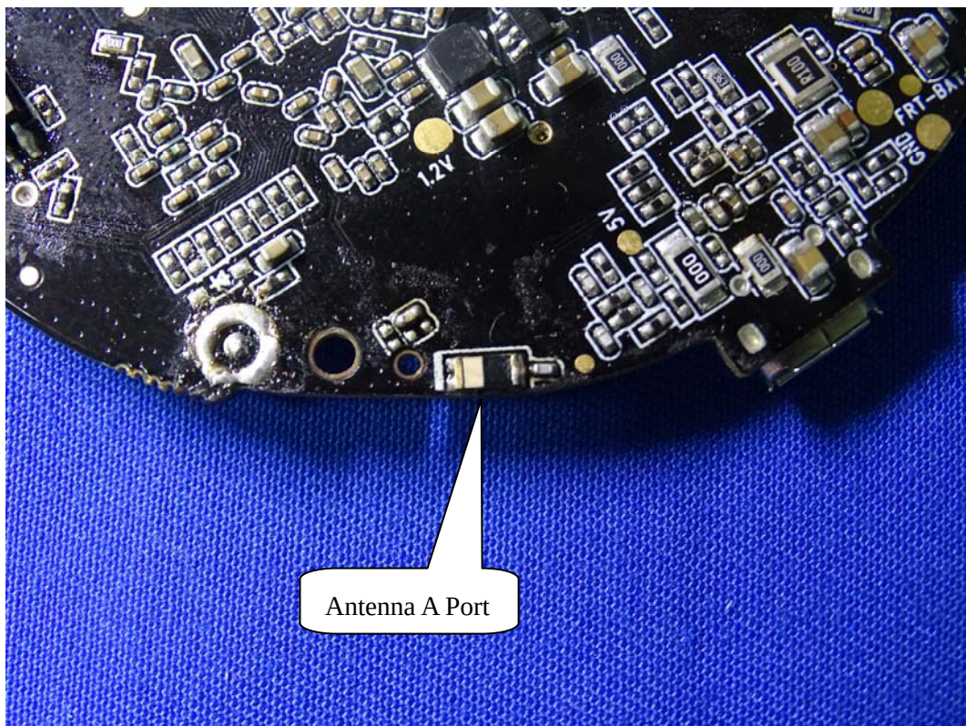
(16) EUT Photo-2.4G Antenna
