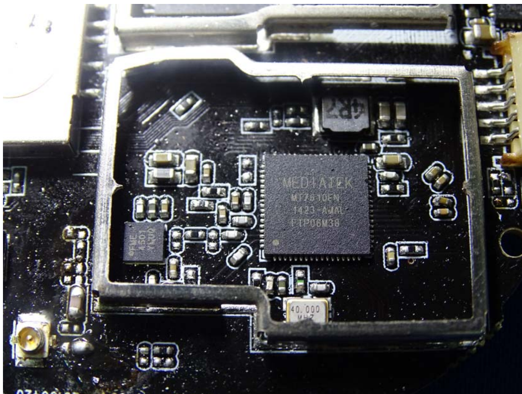
(24) EUT Photo-5G RF Chip
