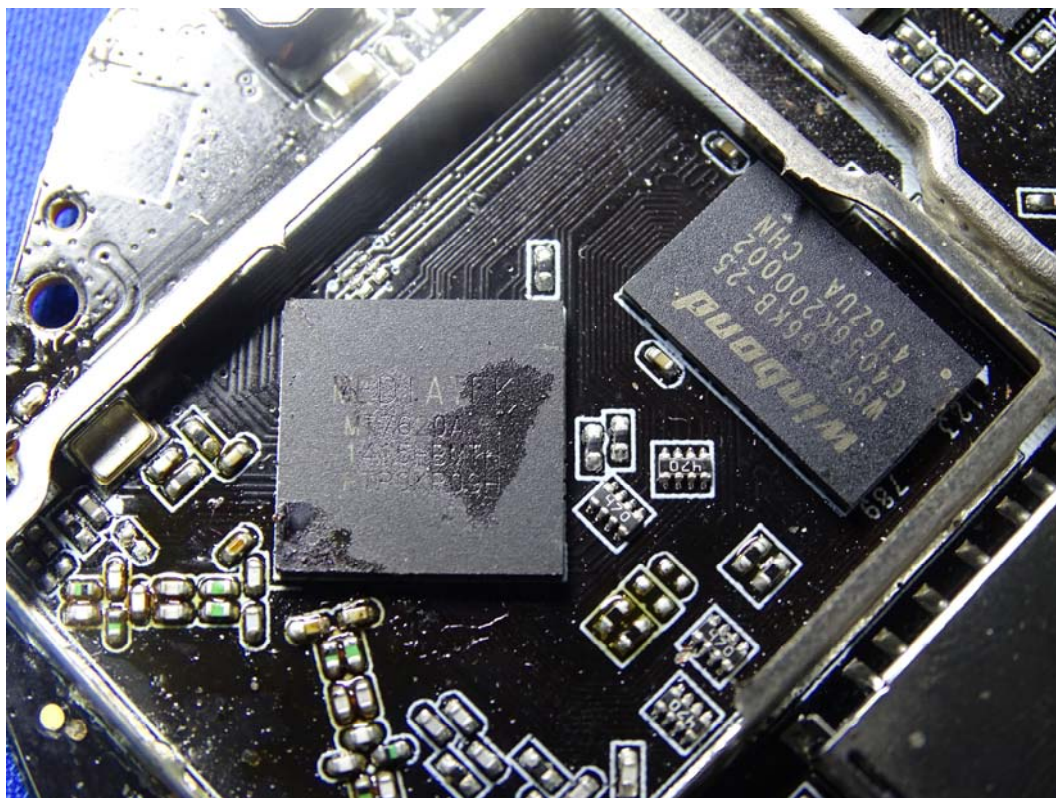
(25) EUT Photo-2.4G RF Chip
