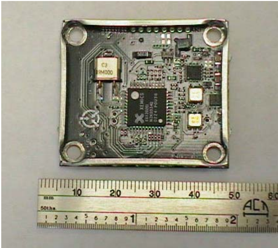
Photo 4. EUT, Top View of TX with Shield Removed
