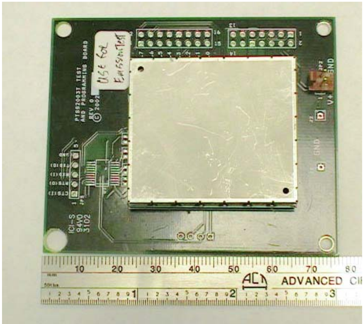
Photo 1. Top View of Interface Board w/ EUT
