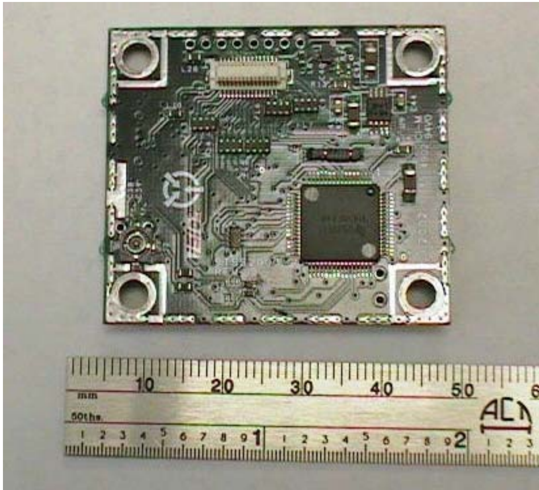
Photo 5. EUT, Bottom View of TX
