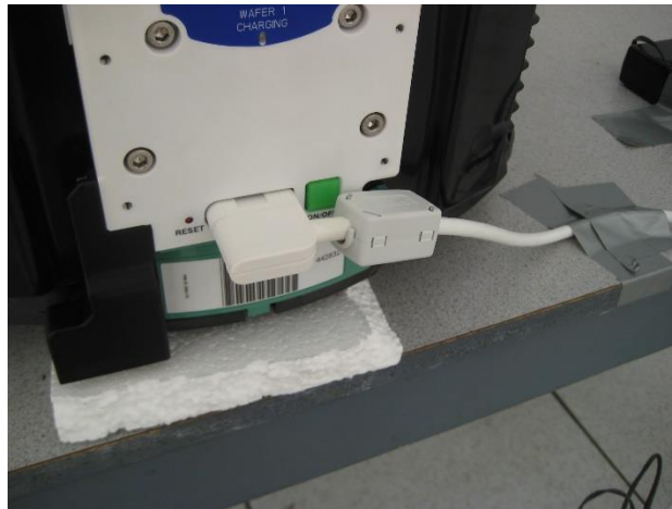
Modification 1: Ferrite, Wurtz electronics, 742.711.32
