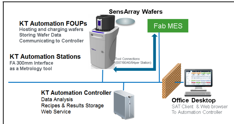
Figure 1-1: KT Automation System Topology
