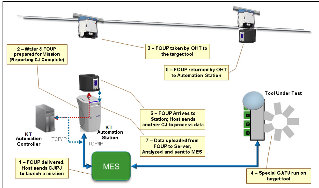
Figure 1-2: KT Automation System Mission Sequence
