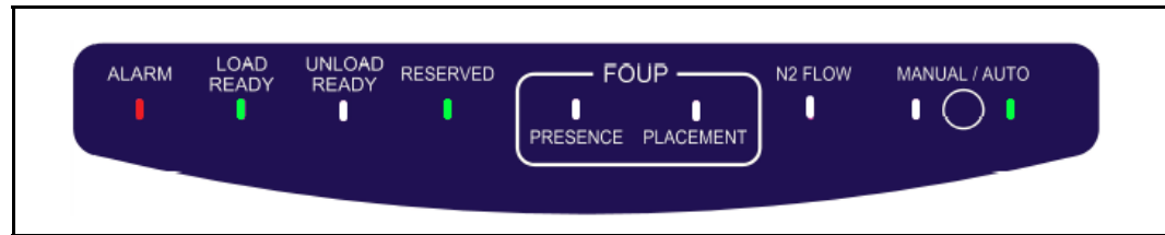
Figure 2-2: KT Automation Station Indicator Panel
