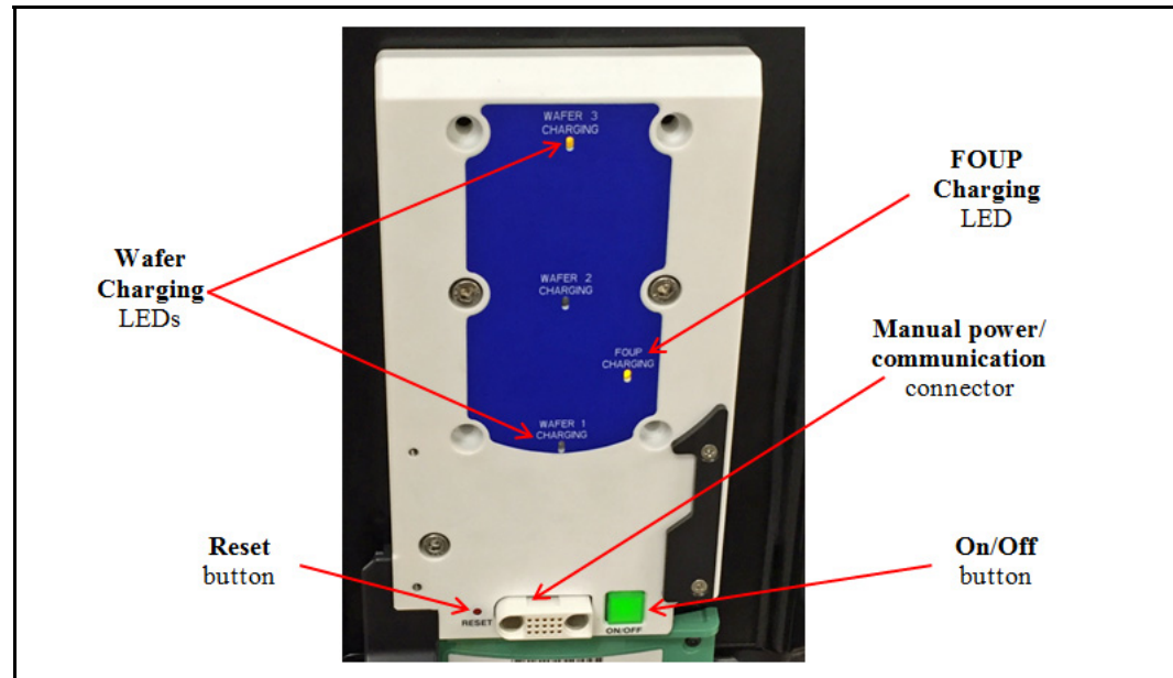
Figure 2-4: KT Automation FOUP Indicators and Controls
