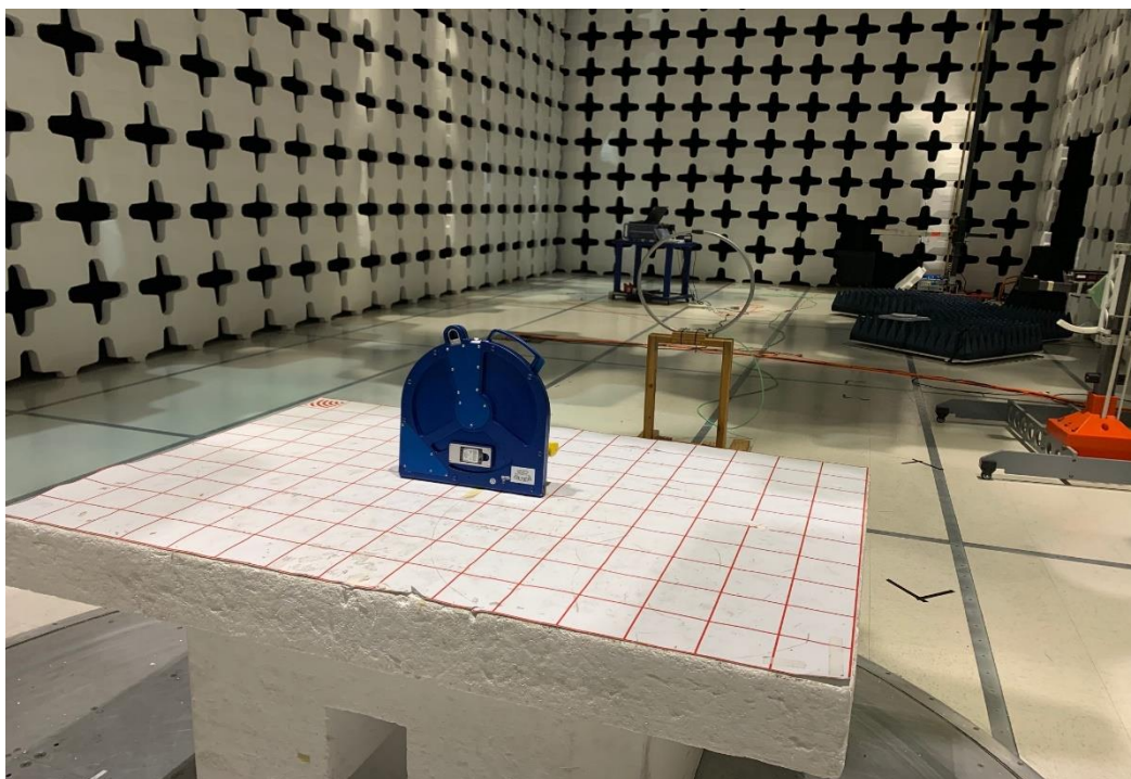
Radiated Emission 9KHz – 30MHz (0 Degree – Rear View)
