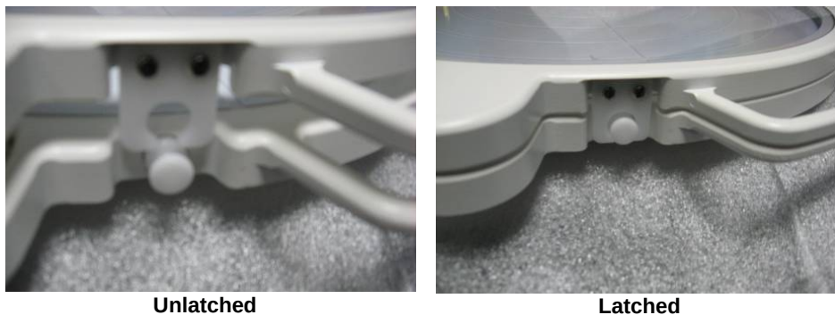
Figure 3-11 Lid Locking Pin
