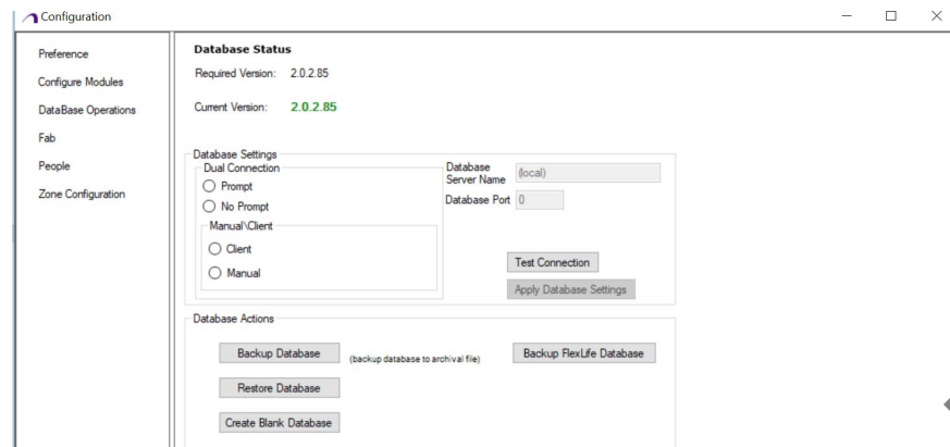
Figure 5-31 Database Operation
