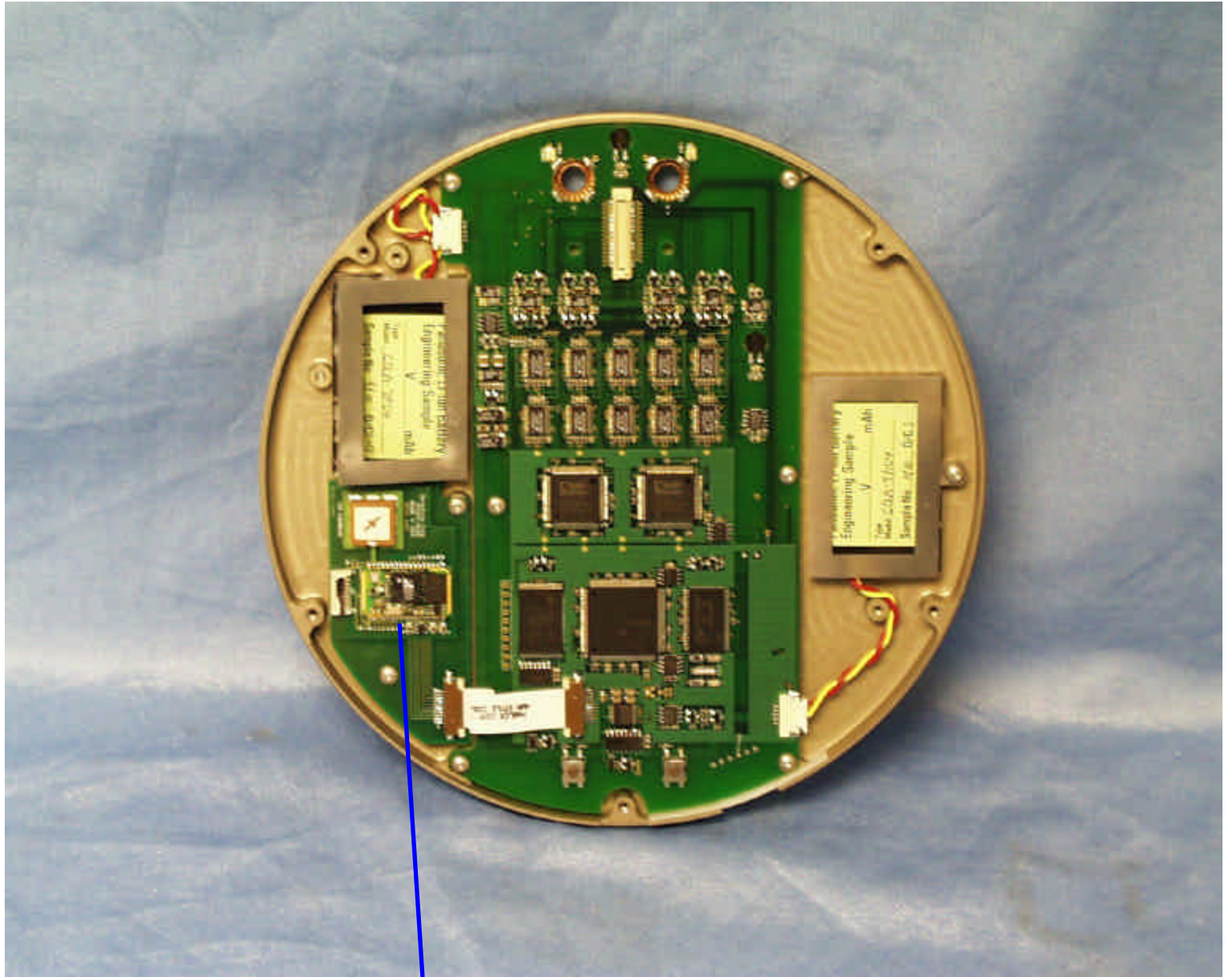
Bluetooth Radio
