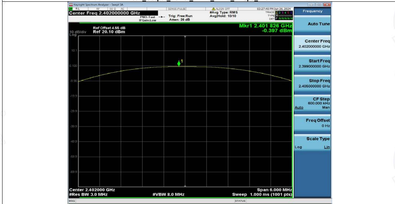
Peak_Output_Power_NVNT_ANT1_1Mbps_2402
