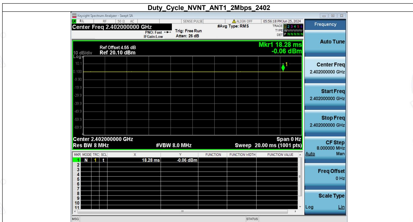
Duty Cycle_NVNT_ANT1_2Mbps_2440
