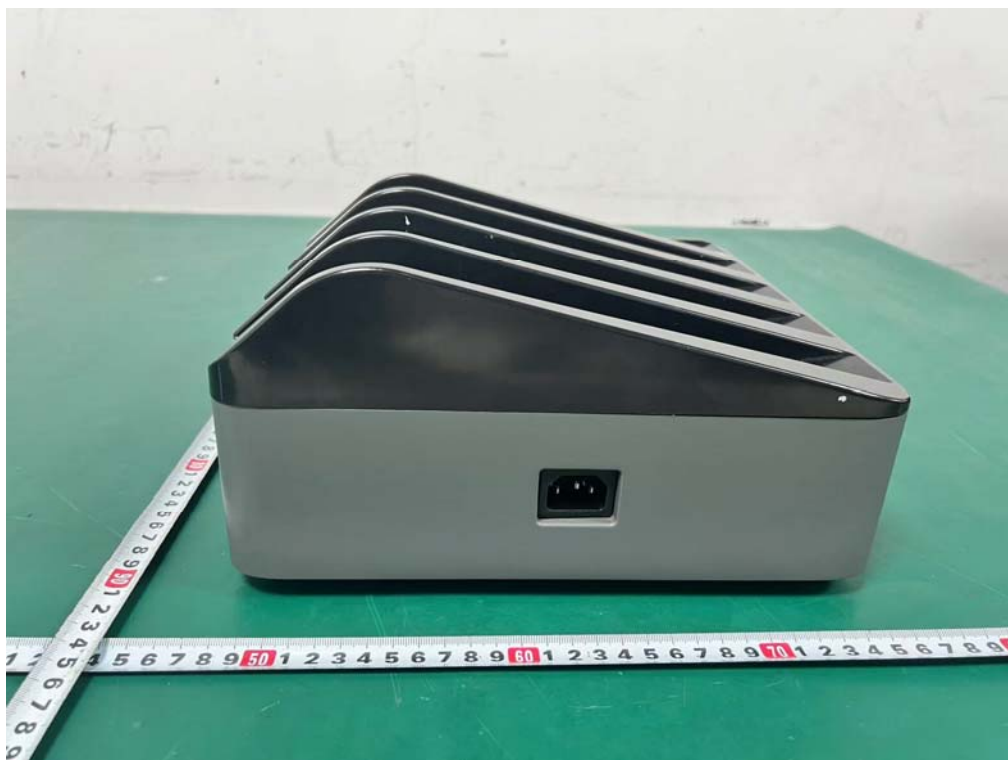
External Photos M/N: ZWL109CHE35
