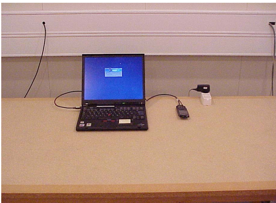
Picture 4 AC powerline conducted emission measurement GSM1900 RX and BT TX + Computer peripherals
