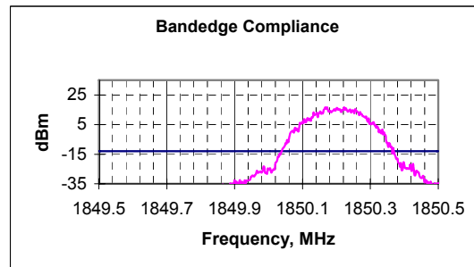
Lower bandedge, channel 512 EGPRS. 3KHz Bw and VBw
