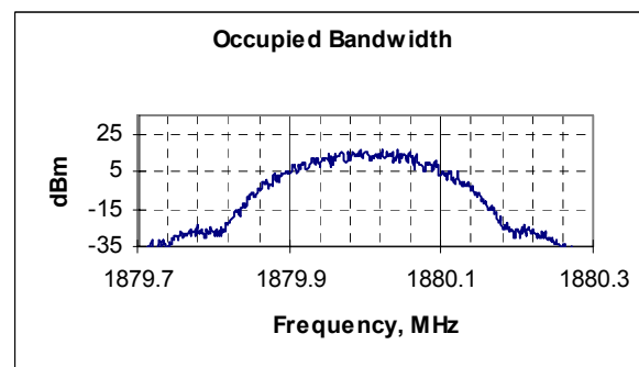
Picture 5. 99% occupied bandwidth, channel 661 EGPRS1900 3KHz Bw and VBw
