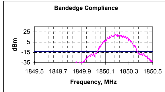
Lower bandedge, channel 512 GSM. 3KHz Bw and VBw
