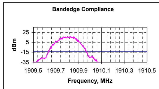
Upper bandedge, channel 810 EGPRS. 3KHz Bw and VBw
