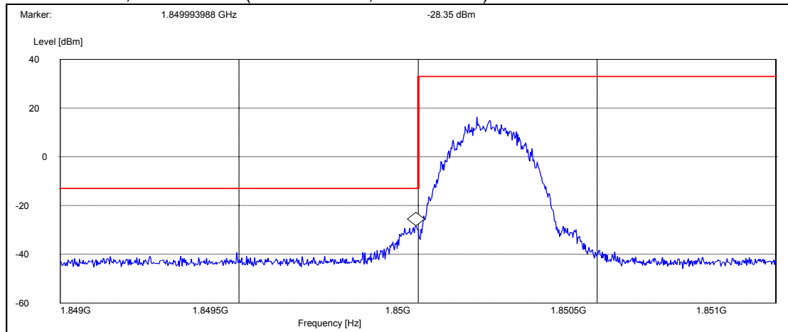
EGPRS mode, channel 512 (Peak detector, RBW: 3 kHz)
