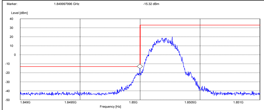
GSM mode, channel 512 (Peak detector, RBW: 3 kHz)
