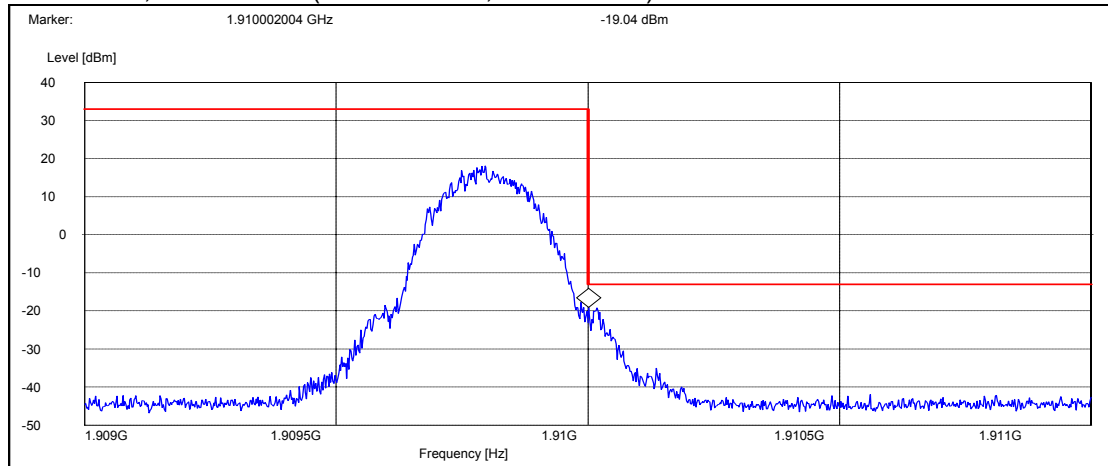
GSM mode, channel 810 (Peak detector, RBW: 3 kHz)
