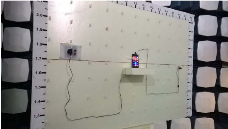
Picture 2. FCC Part 15B Radiated emissions
