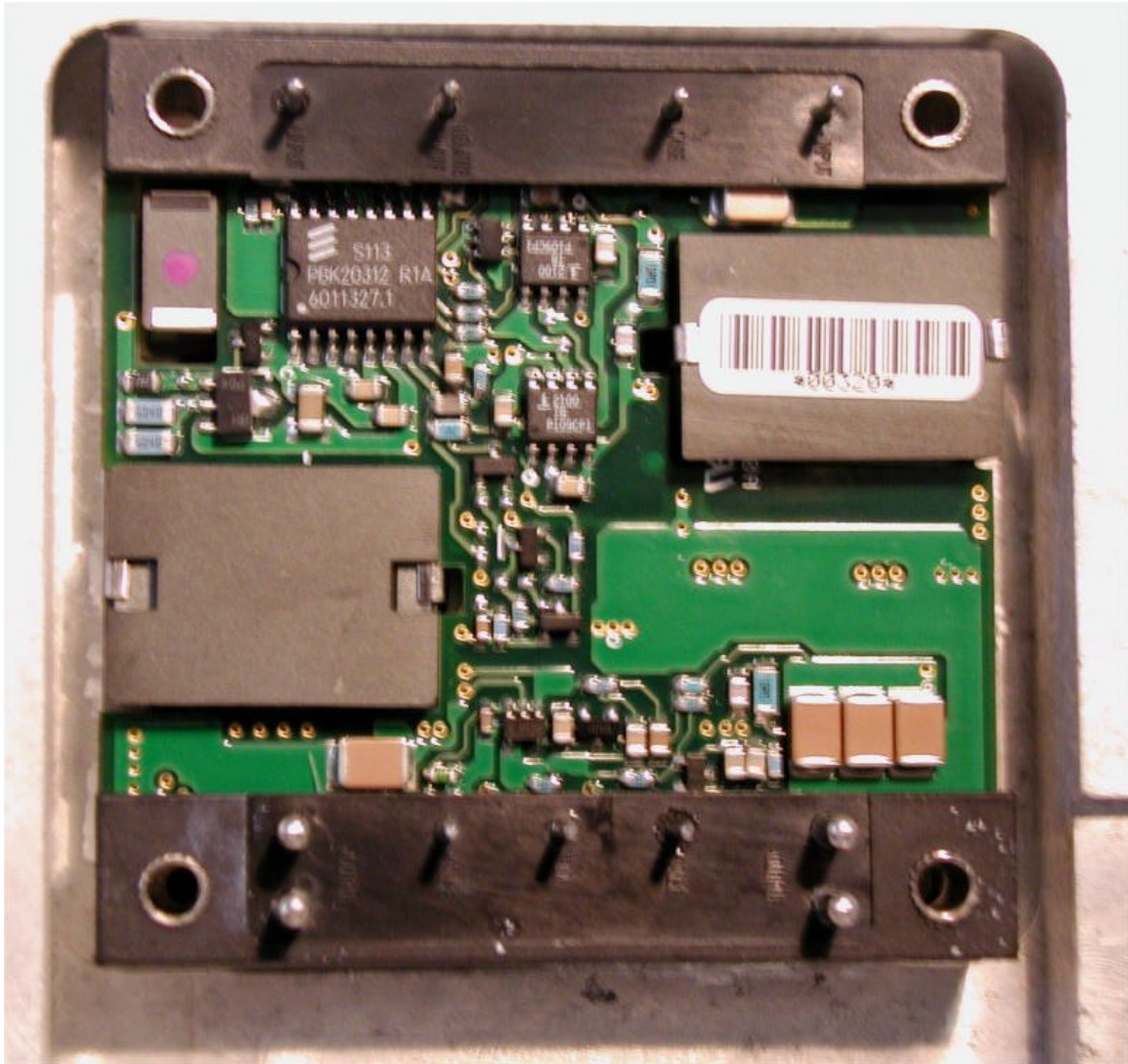
PLK 4316 PIT DC CONVERTER COMPONENT SIDE
