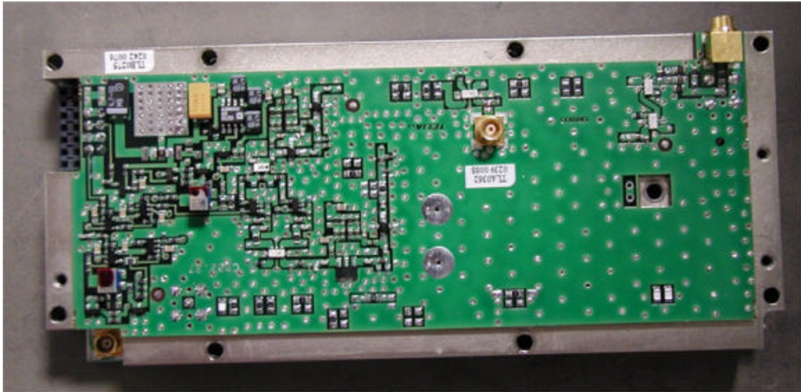
TLA 0362 UPPER SIDE
