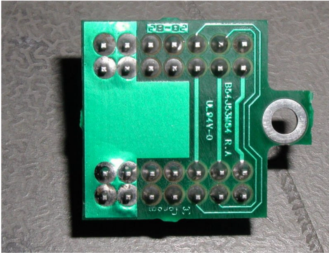
INTERCONNECTION BOARD FOIL SIDE
