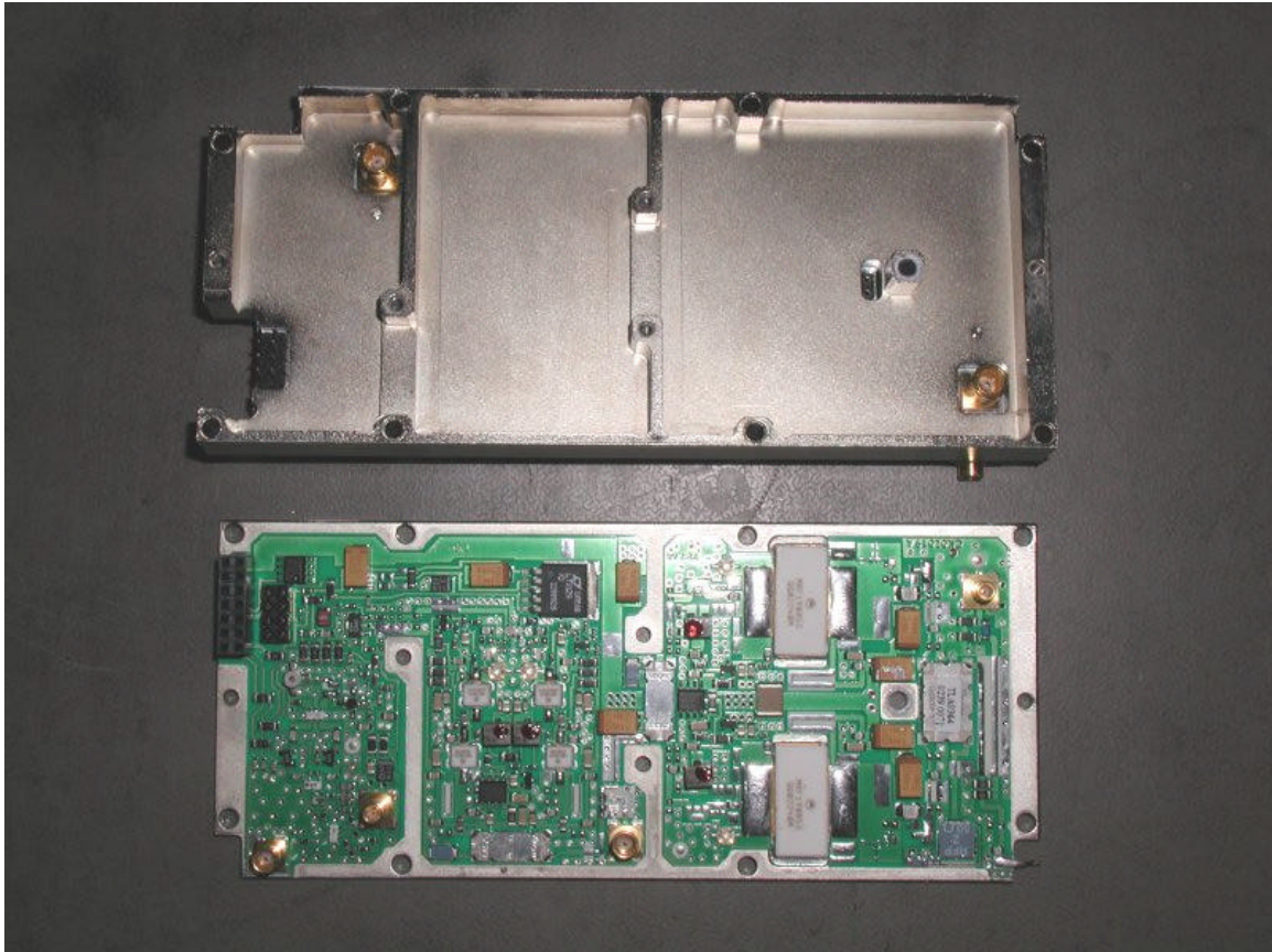
TLA 0362 LOWER SIDE / TLA 0364 COMPONENT SIDE
