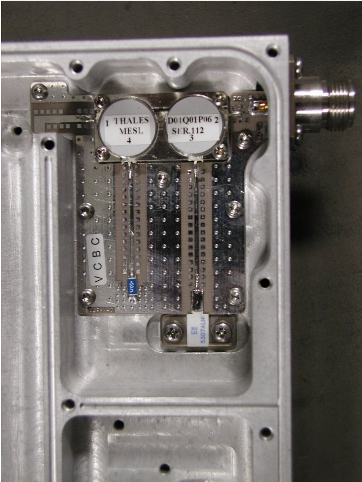
OUTPUT CIRCUIT COMPONENT SIDE
