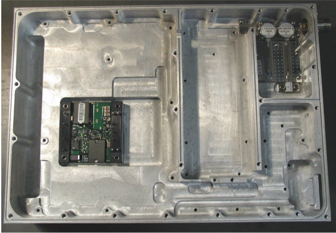
DRIVER AND TLA BOARDS REMOVED
