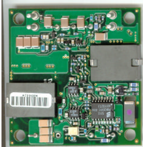
DCDC SIDE 1
