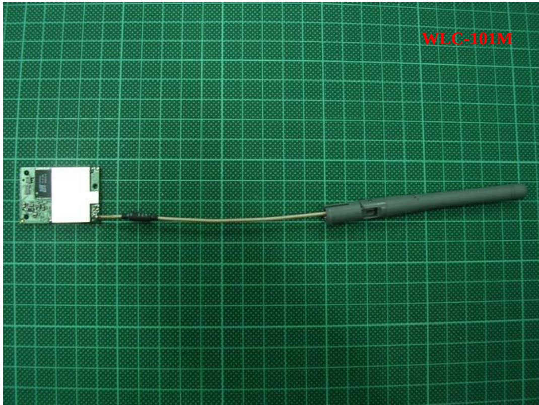
Photo 2: Exterior photo of EUT with antenna 2
