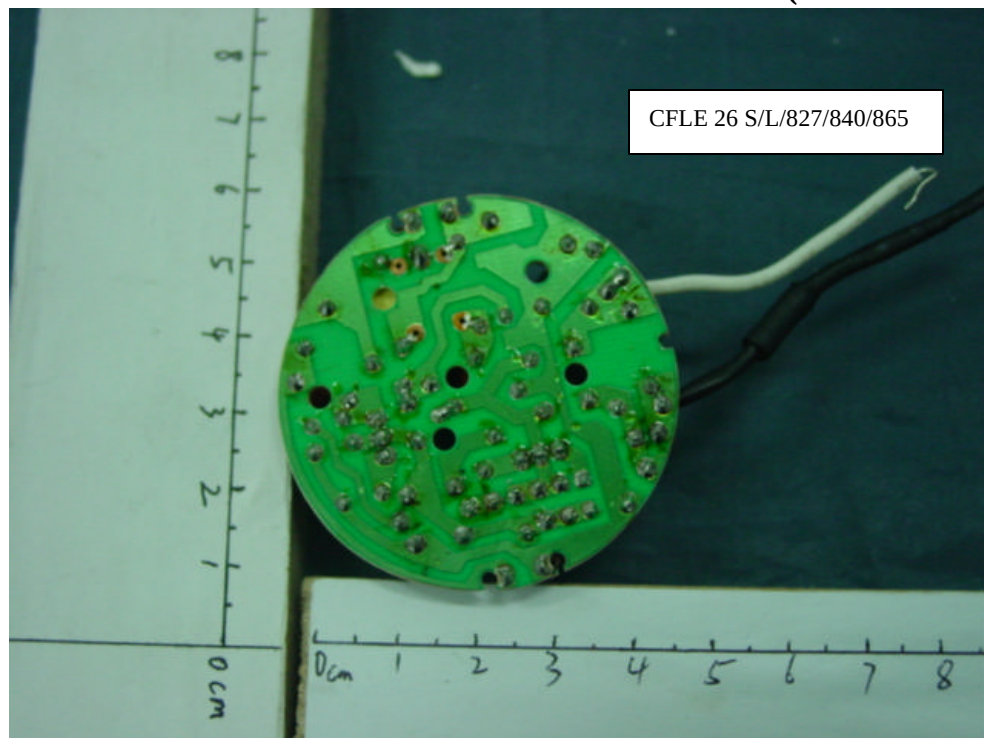
FIGURE 12 Energy Saving Lamp Main Board (Soldered Side)
