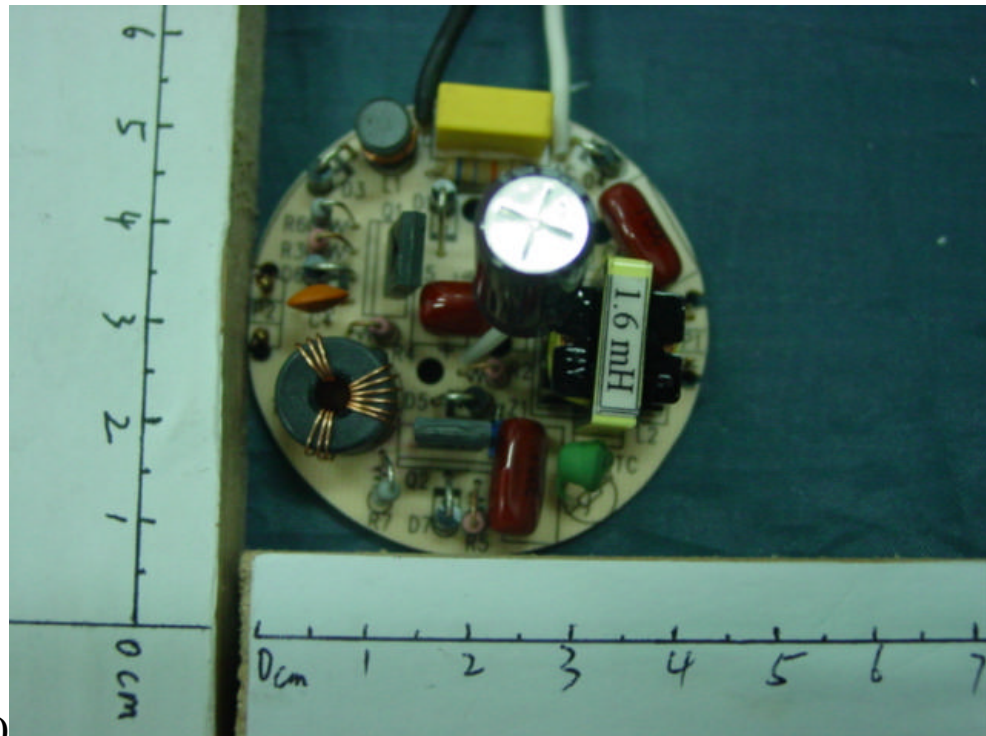
FIGURE 4 Energy Saving Lamp Main Board (Soldered Side)
