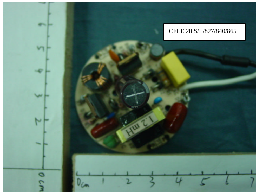
FIGURE 8 Energy Saving Lamp Main Board (Soldered Side)
