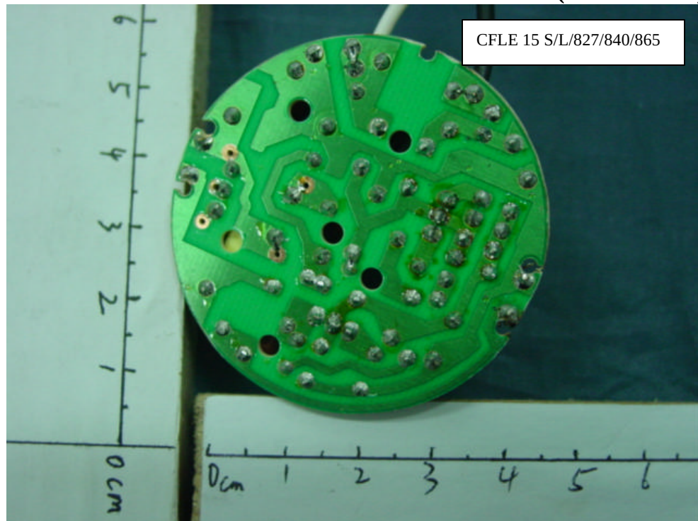
FIGURE 5 Energy Saving Lamp Main Board (Component Side)
