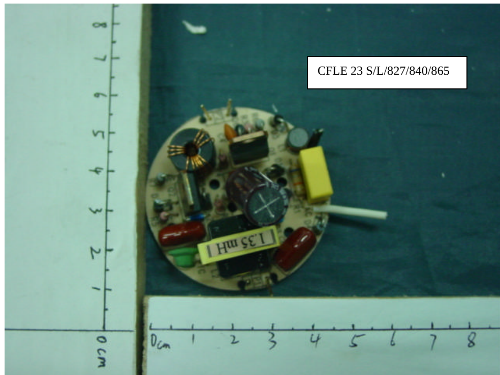
FIGURE 10 Energy Saving Lamp Main Board (Soldered Side)
