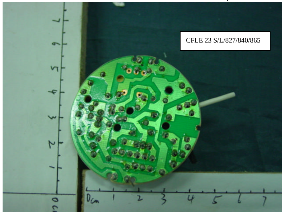
FIGURE 11 Energy Saving Lamp Main Board (Component Side)
