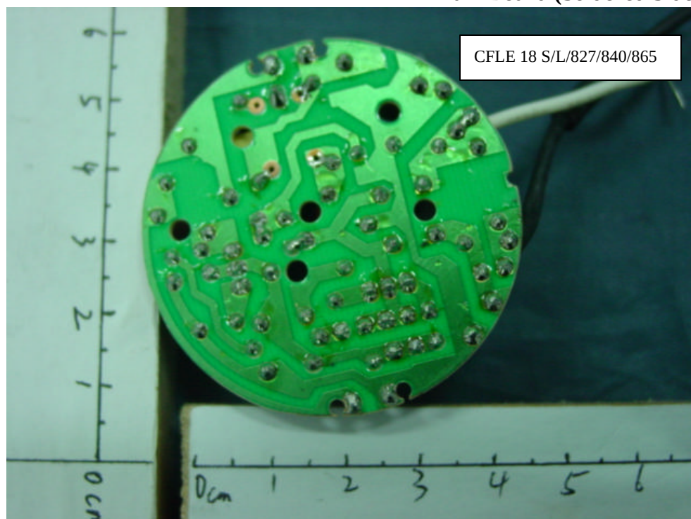
FIGURE 6 Energy Saving Lamp Main Board (Soldered Side)
