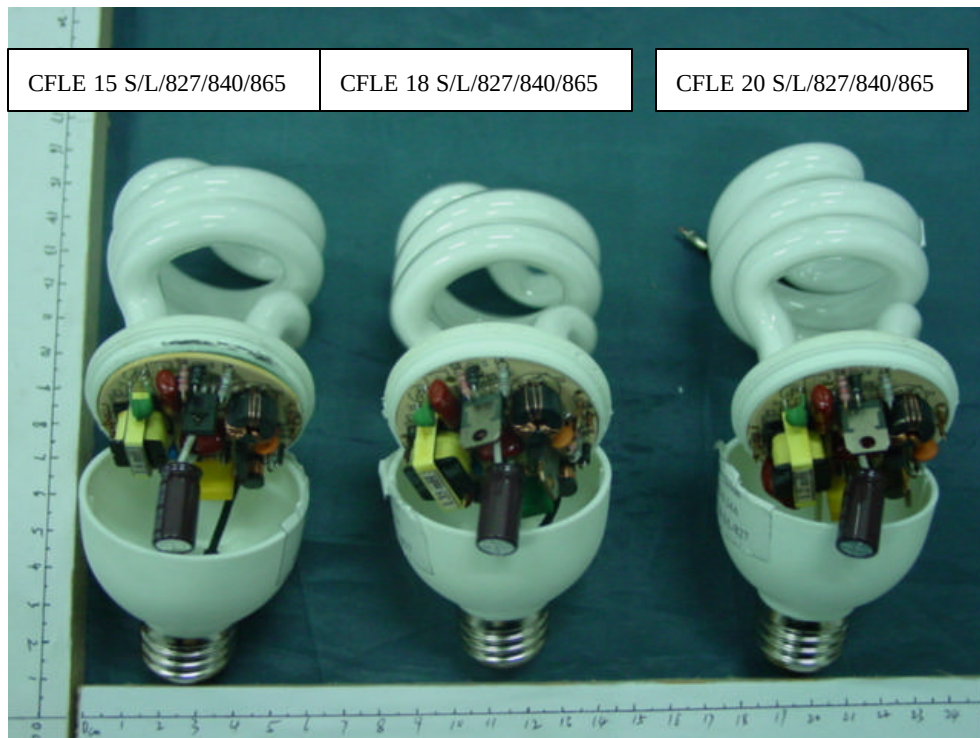
FIGURE 2 Energy Saving Lamp Cover Removed
