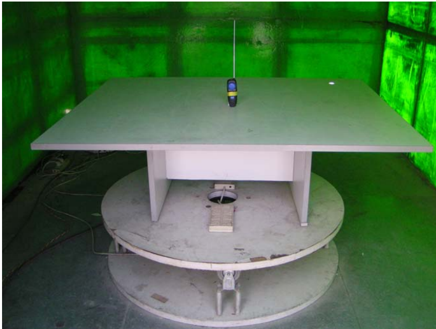
Radiated Emission – Stand View
