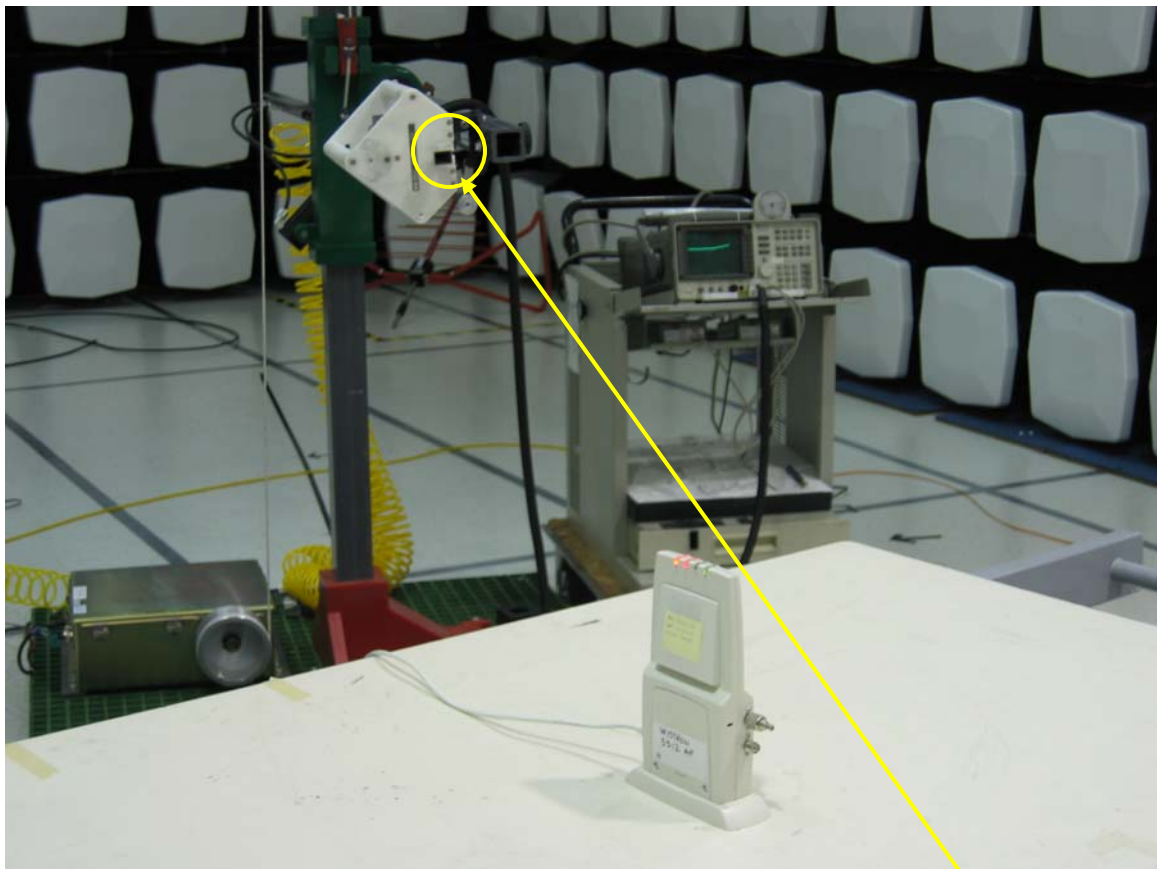
26-40GHz Horn antenna
