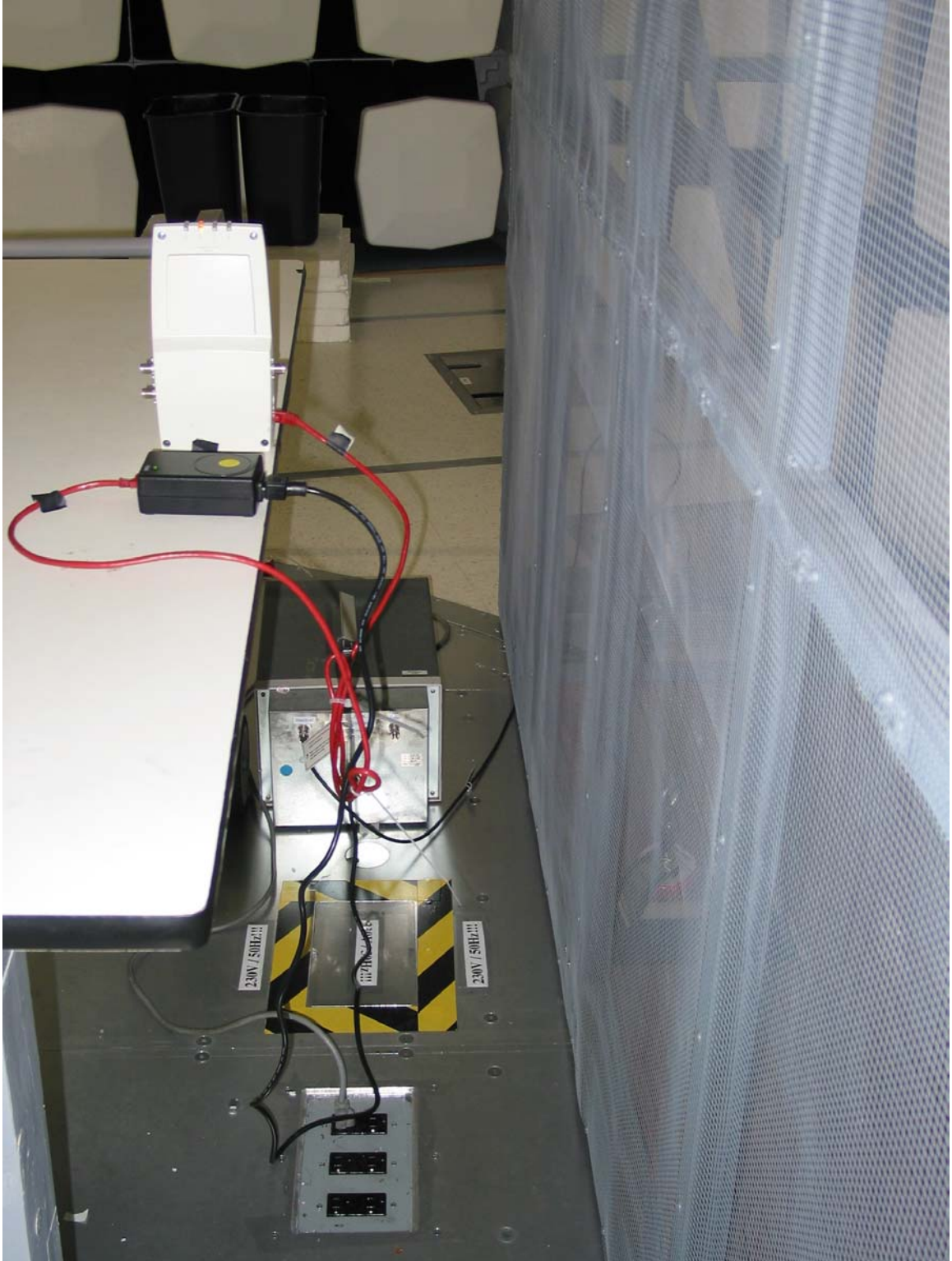
AC Line Conducted Emissions
