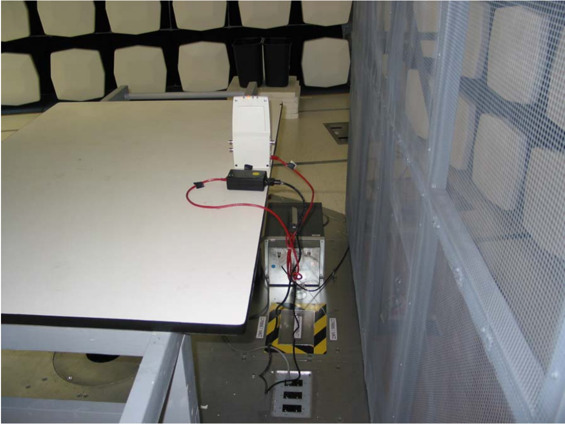
AC Line Conducted Emissions
