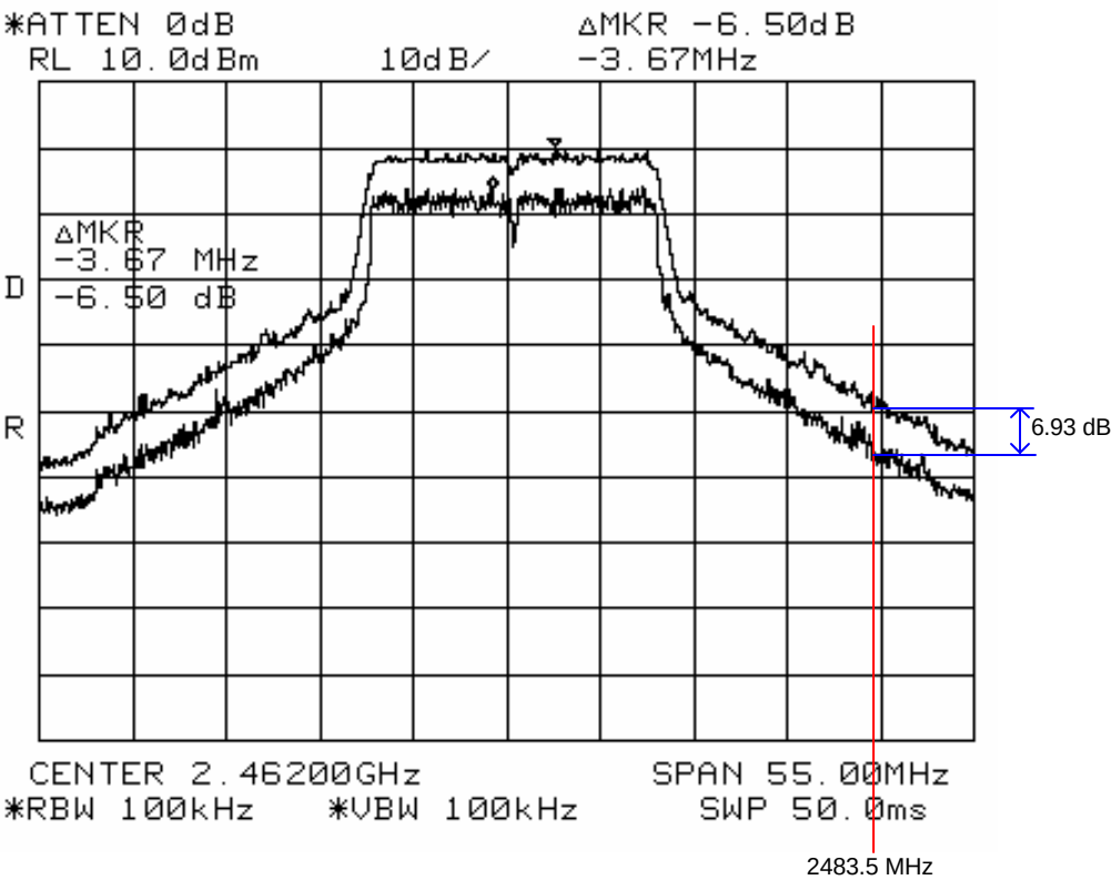
802.11 G 2483.5 MHz BW Delta Measurement
