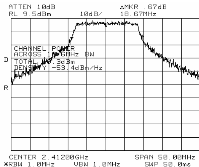
99% Channel power, 802.11 G Channel 1
