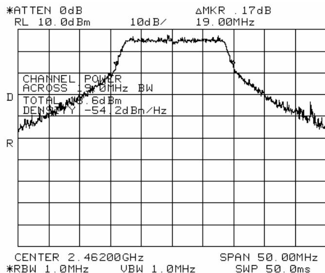
99% Channel power, 802.11 G Channel 11
