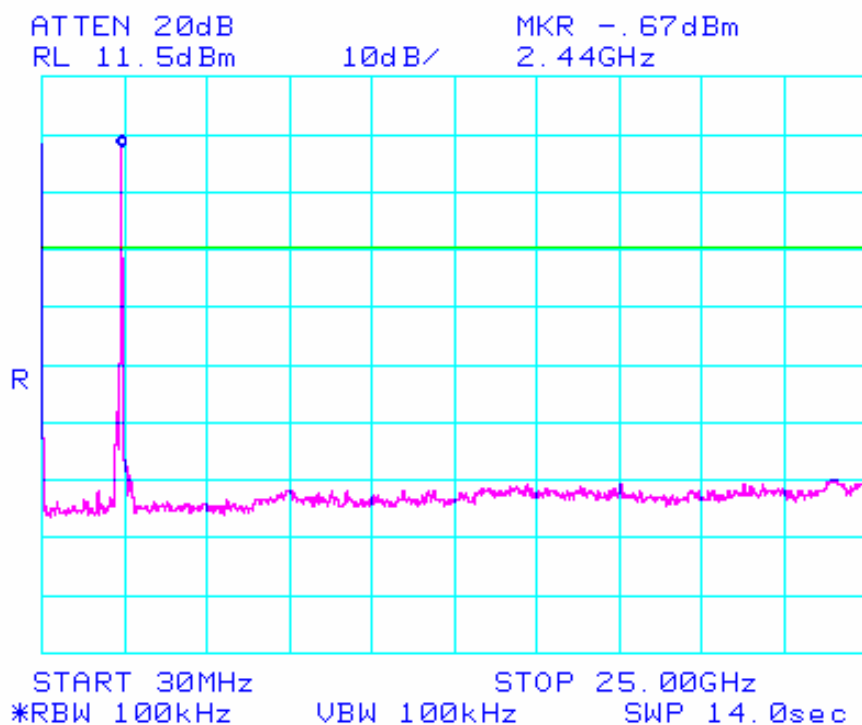
OOB Emissions, Transmit on Channel 6 (2437MHz)
