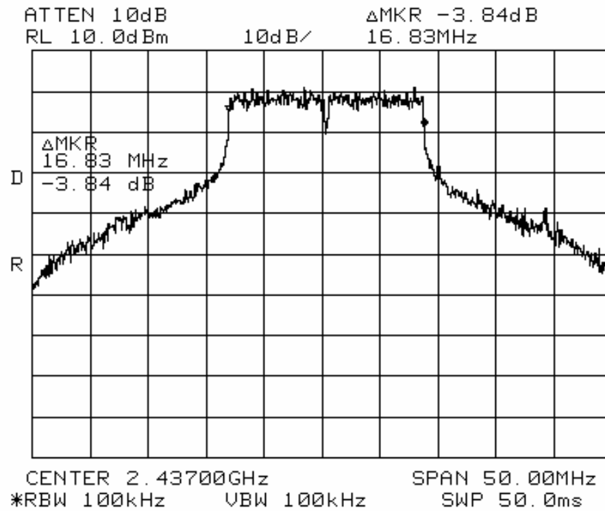
6 dB BW, Channel 6 , 2437 MHz, 802.11 G
