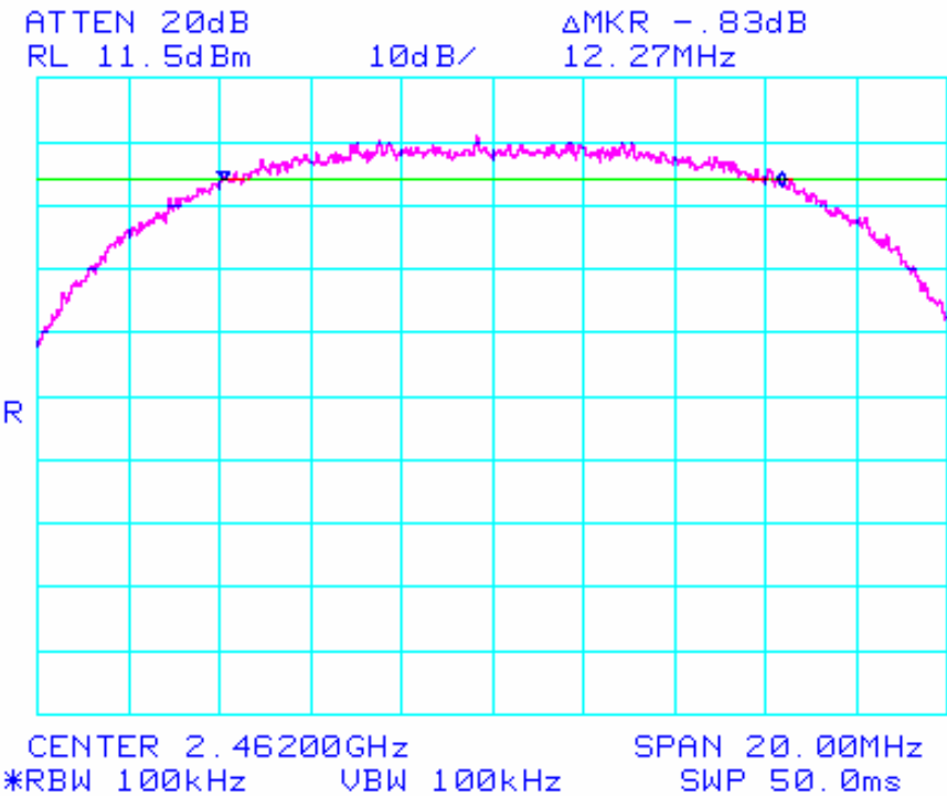
6 dB BW, Channel 11, 2462 MHz, 802.11 B
