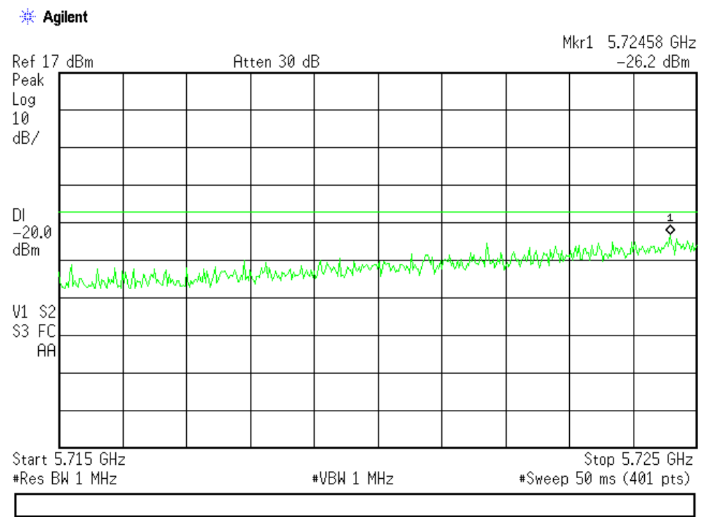
Plot of the 5,725 GHz lower band edge showing the peak @ -26.2dBm
