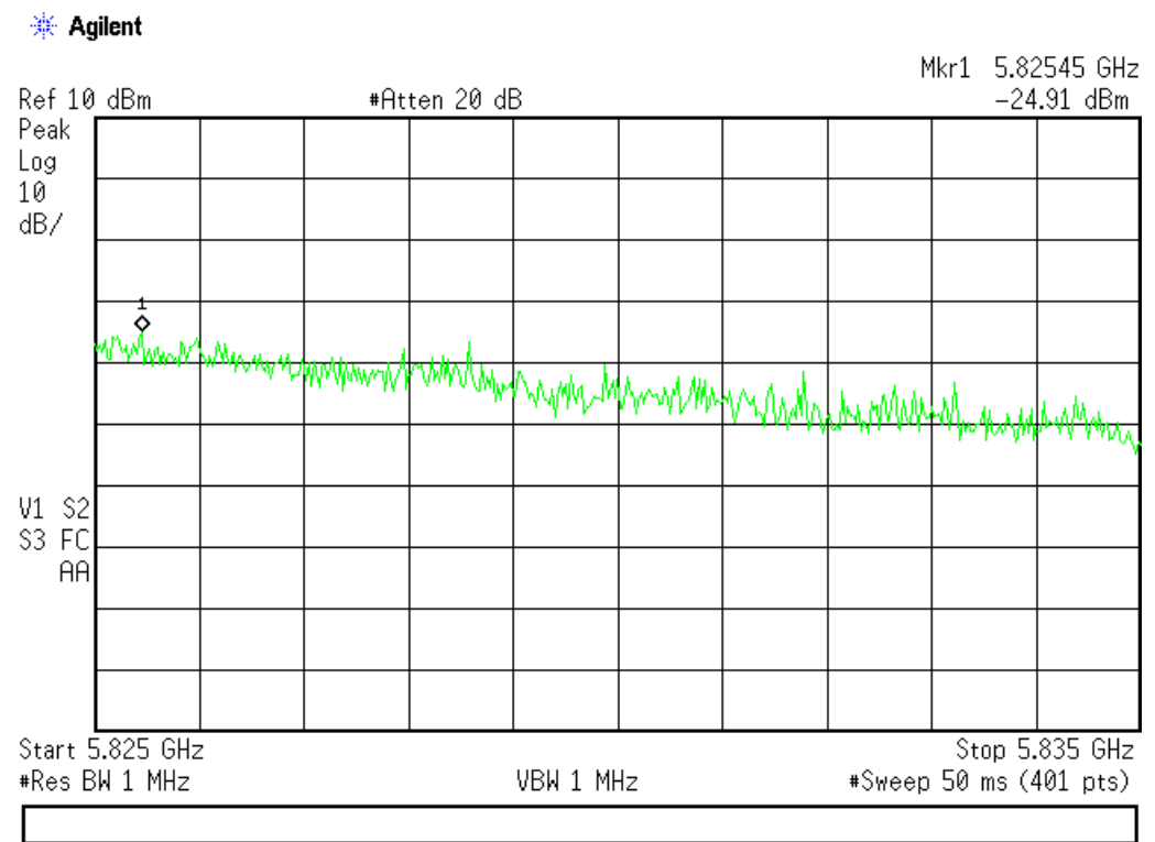
Plot of the 5,825 GHz upper band edge showing the peak @ -24.91dBm
