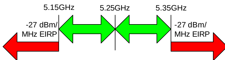
Out Of Band Spurious Emissions Limits
