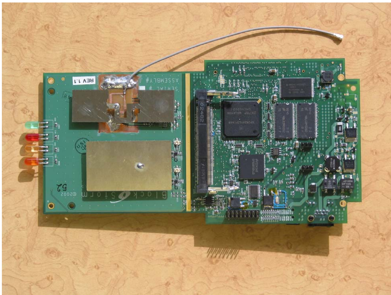
Main PCB, Side 1 removed from housing showing 802.11 A expansion slot
