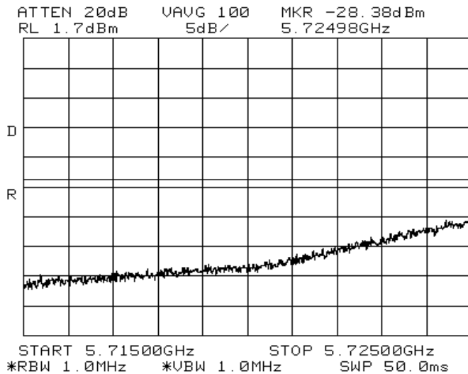
Plot of the 5,725 GHz lower band edge showing the peak @ -28.38dBm
