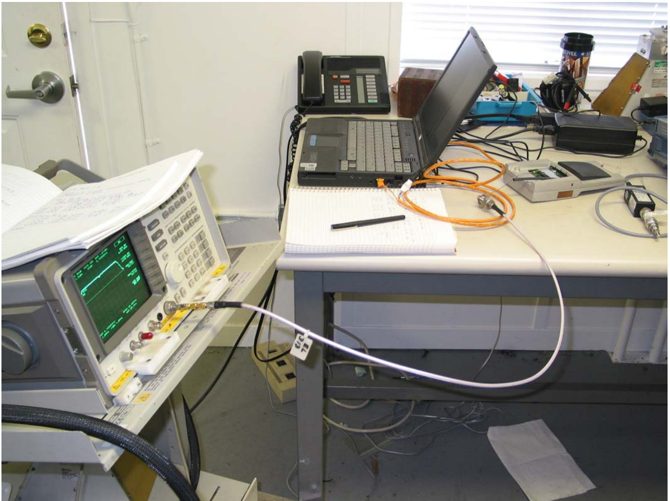
RF Conducted tests bench setup
