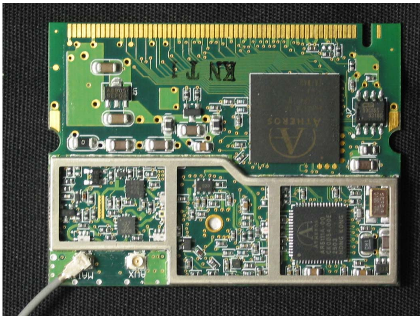
802.11 module, shields removed
