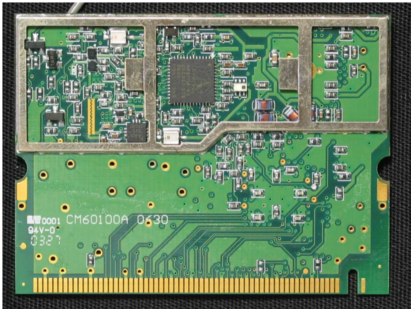
802.11 module, shields removed, rear
