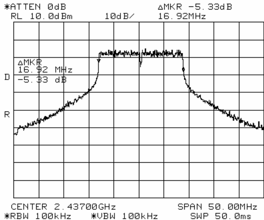
6 dB BW, Channel 6 , 2437 MHz, 802.11 G
