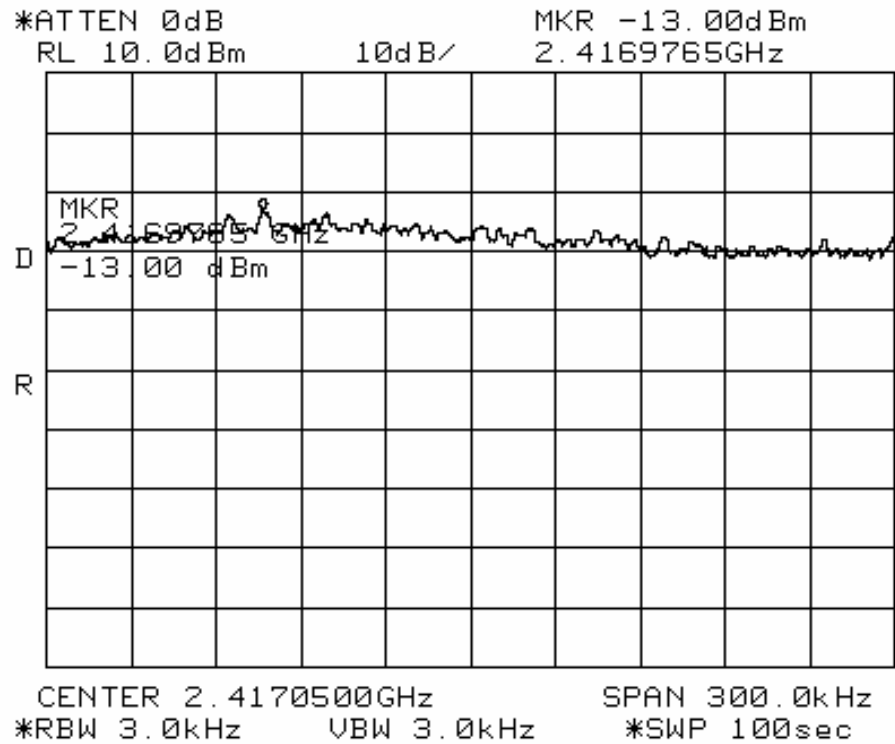
Power Spectral Density, 802.11 G, LOW Channel, 2412MHz
