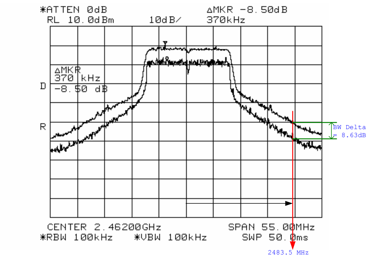
2483.5 MHz BW delta measurement
