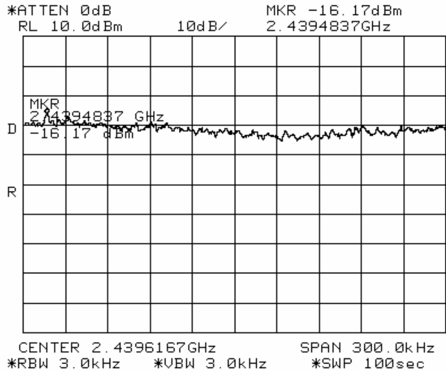
Power Spectral Density, 802.11 G, MID Channel, 2437MHz
