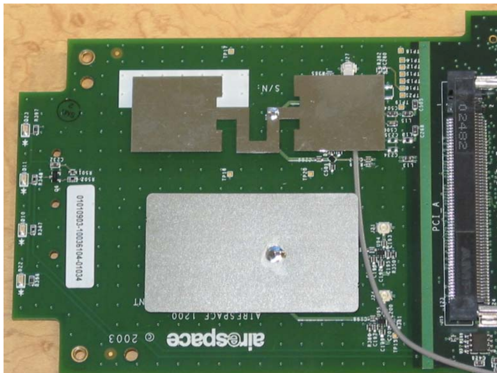
Antenna detail A side
