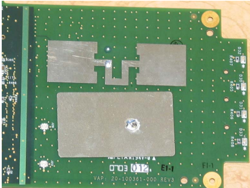
Antenna detail, B side
