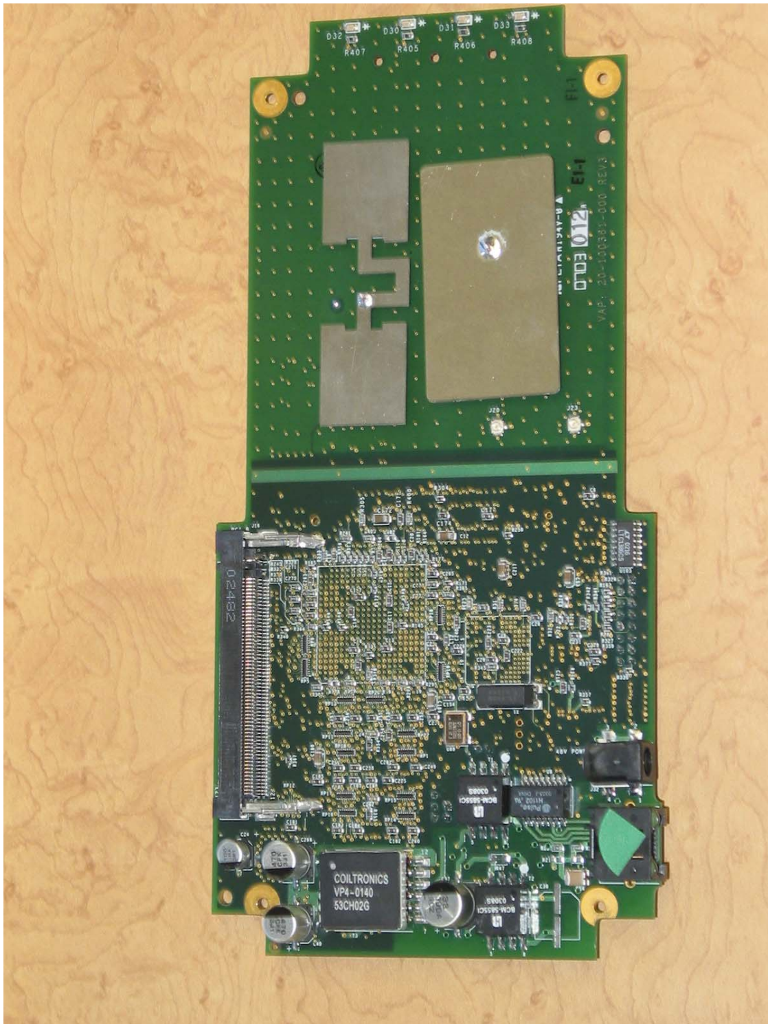
1200B Circuit card removed, PCI module removed, B side
