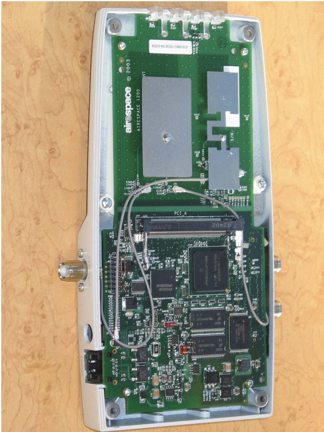
1200B Card, A side
