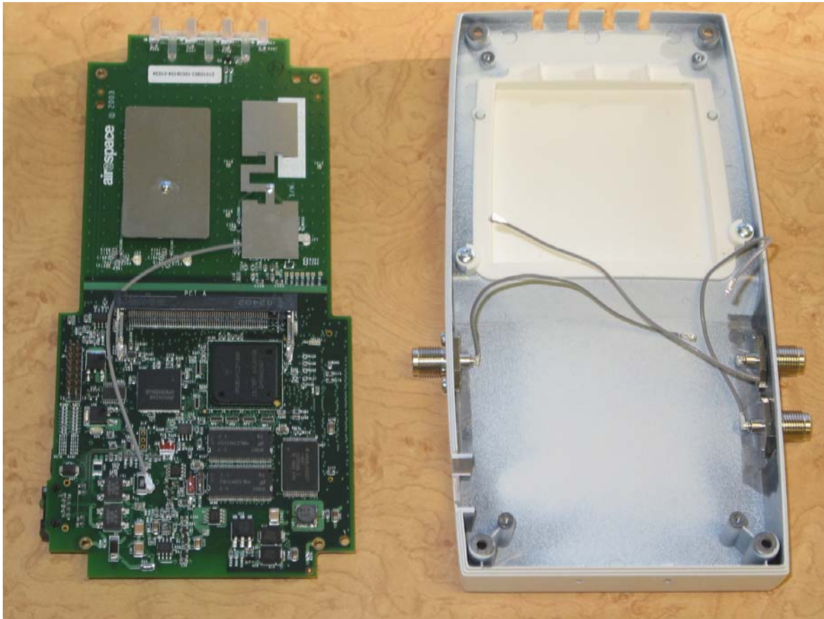
1200B, Card removed, A Side shown
