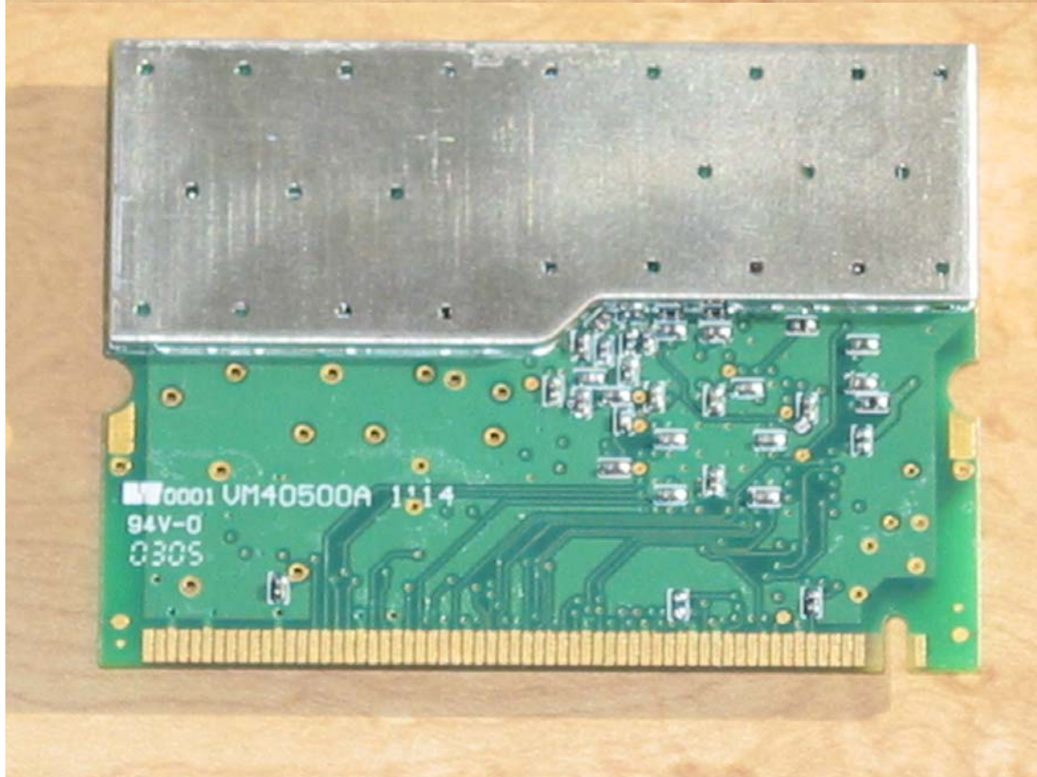
Mini PCI card, cover removed back
