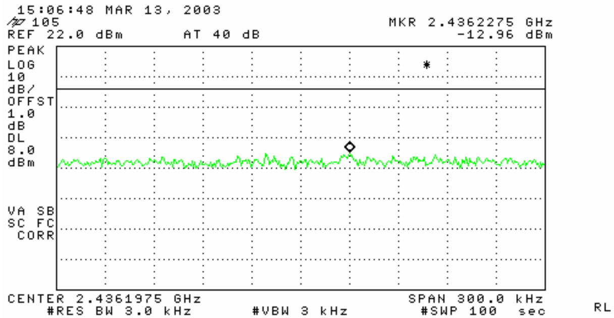
Power Spectral Density, MID Channel, 2437MHz
