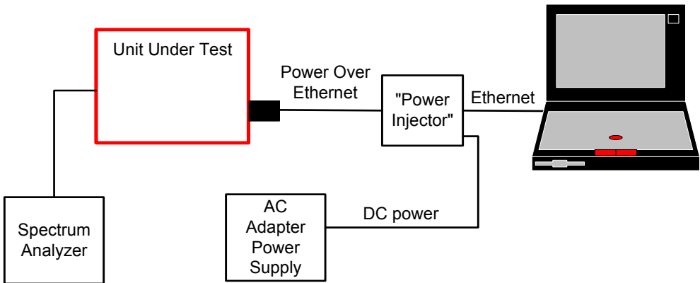
Basic Conducted RF Bench Test Setup
