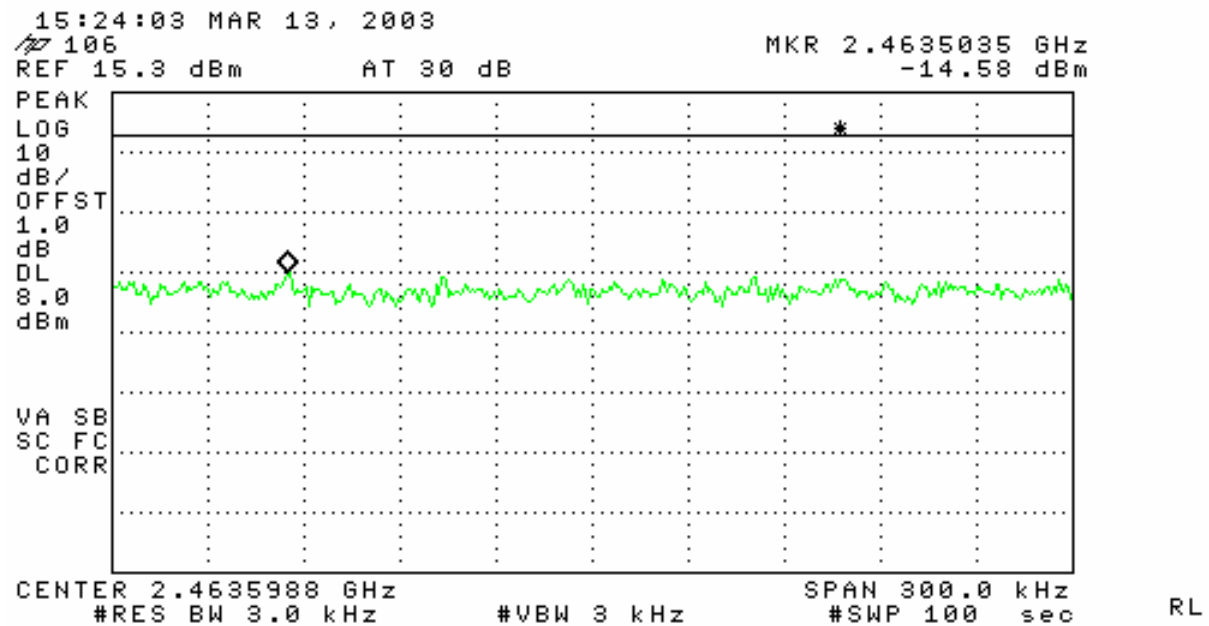
Power Spectral Density, HIGH Channel, 2462MHz
