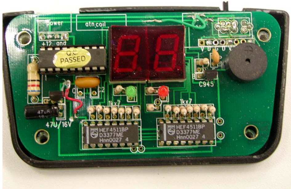
Internal Photo - 2
