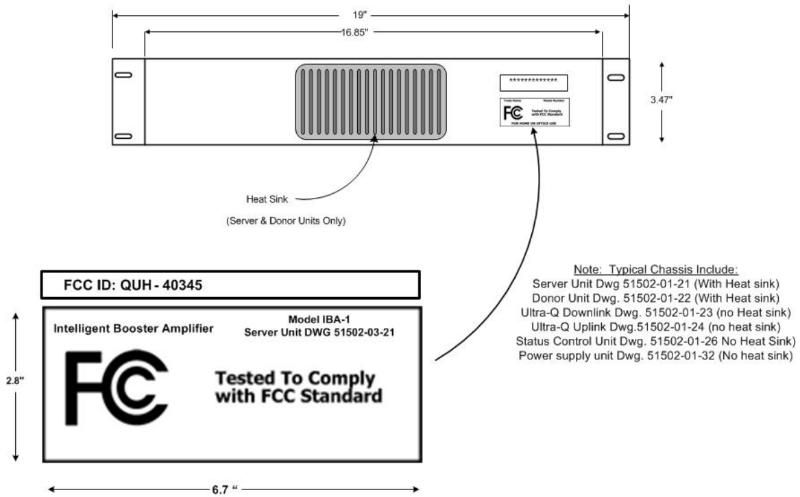
Figure 4A Typical FCC Label Placement Detail
