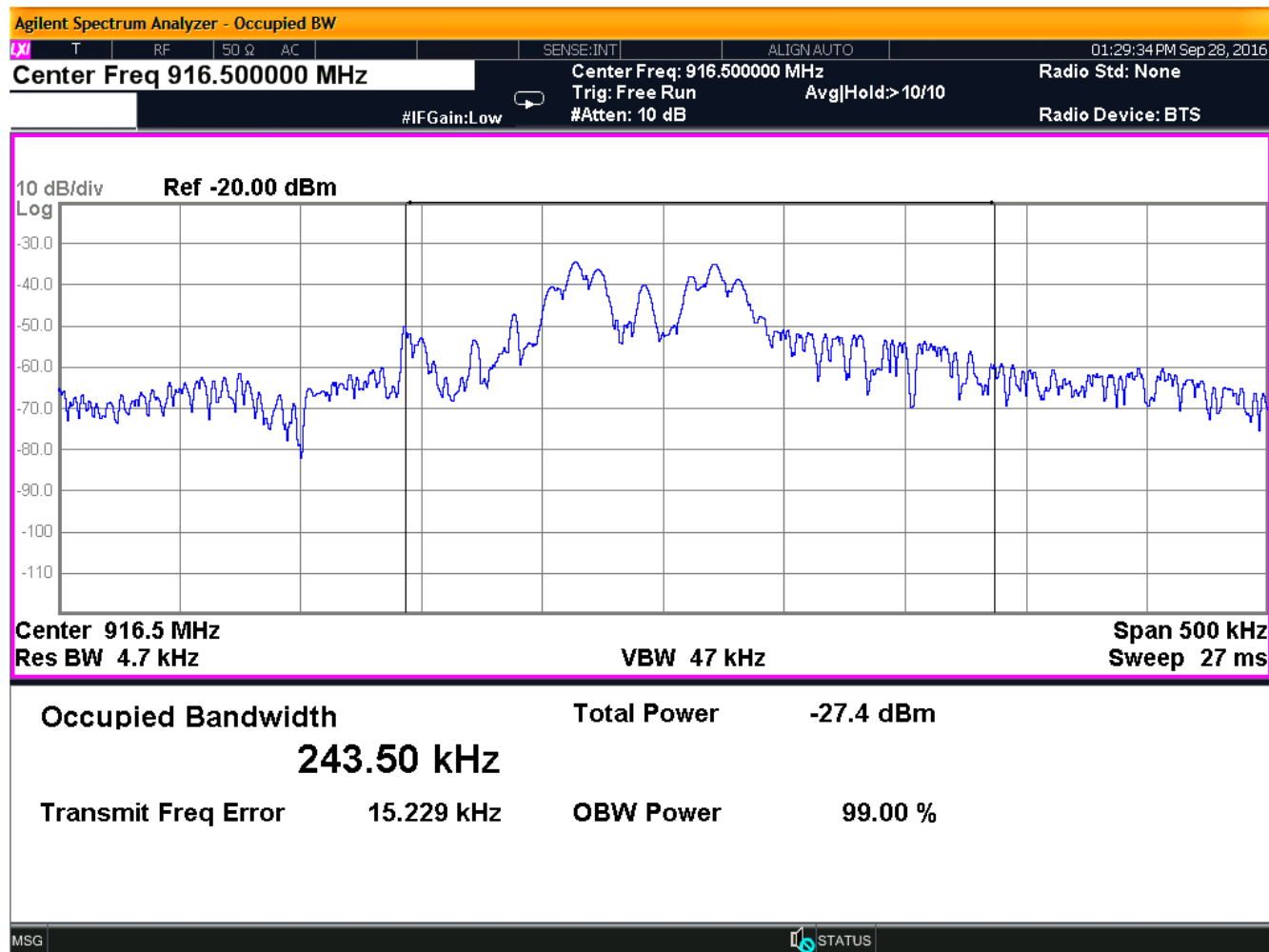
Figure 8: Occupied Bandwidth 99%
