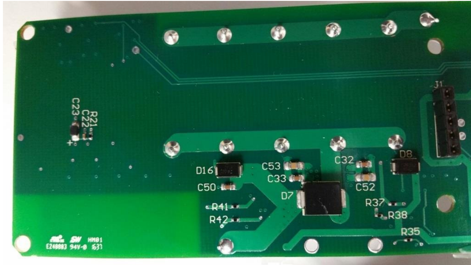
Magnetic Field Generator-Internal Photo Generator/Receiver Board-Bottom View (pt. 1)
