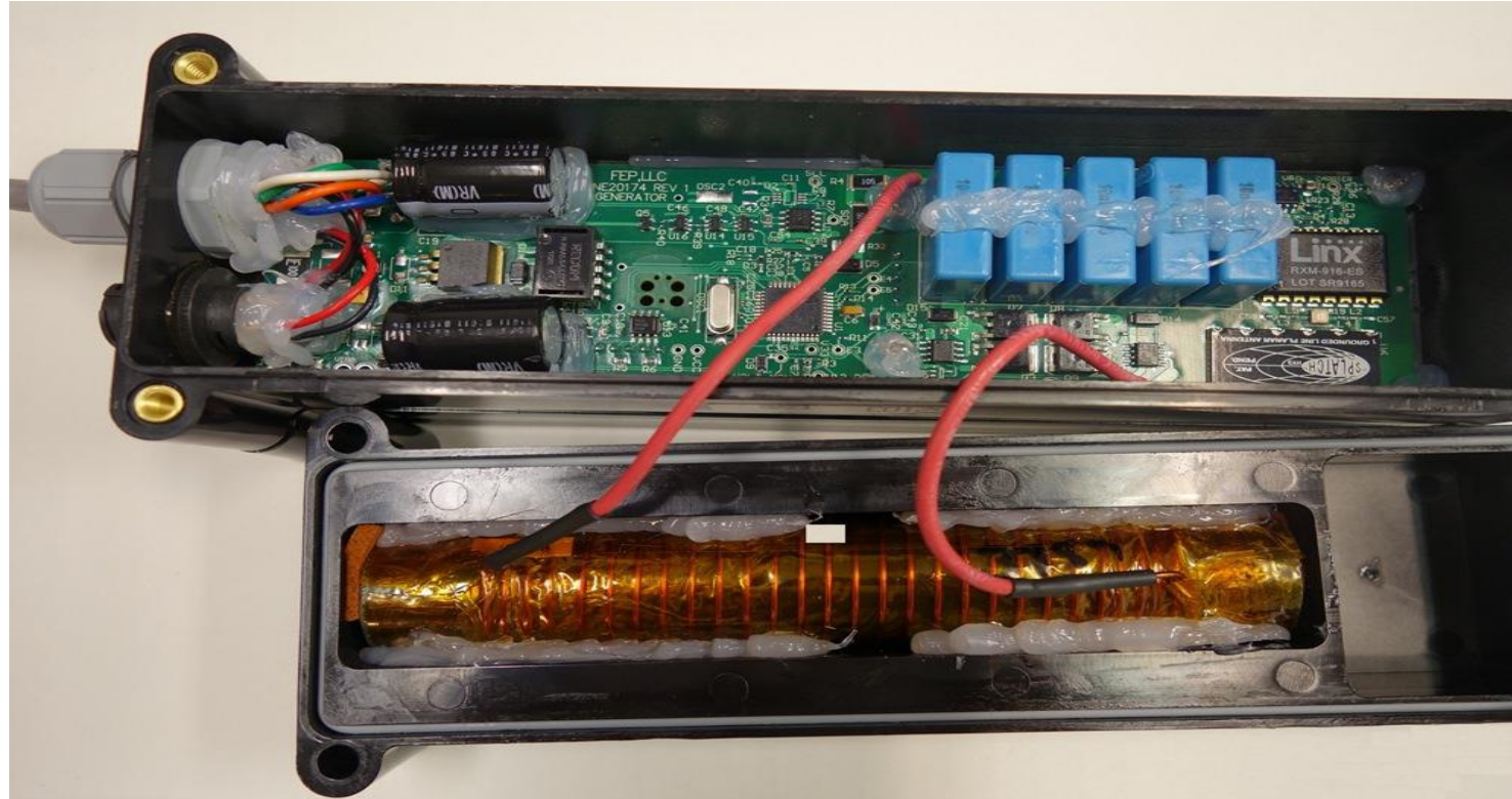
Magnetic Field Generator-Internal Photo Open Ferrite and Middle Housings Circuitry and Wire/Inductor
