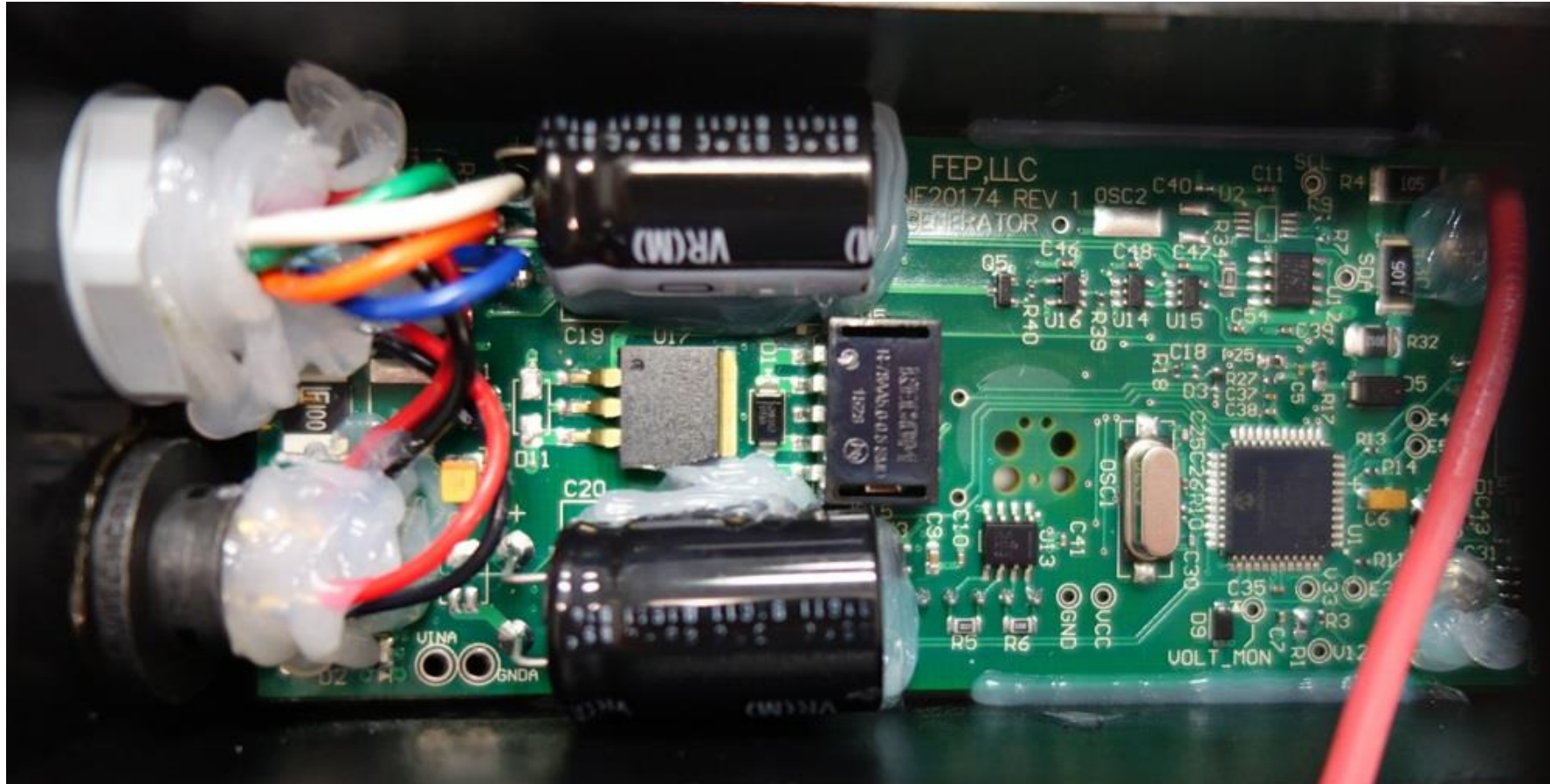
Magnetic Field Generator-Internal Photo Generator/Receiver Board-Top View (pt. 2)
