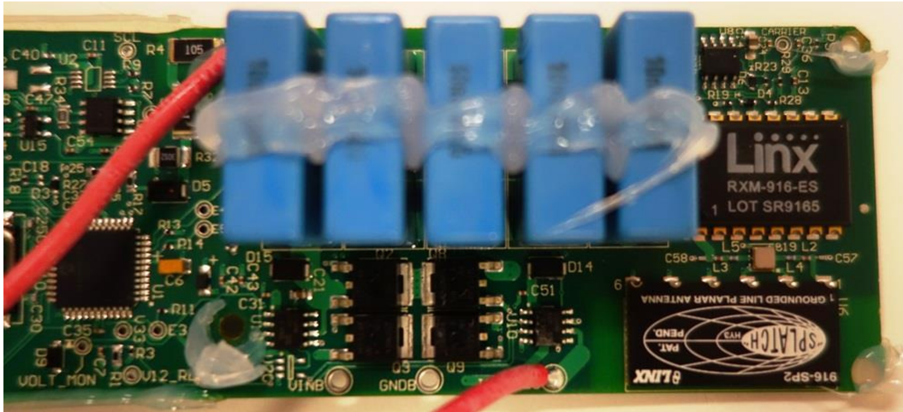
Magnetic Field Generator-Internal Photo Generator/Receiver Board-Top View (pt. 1)
