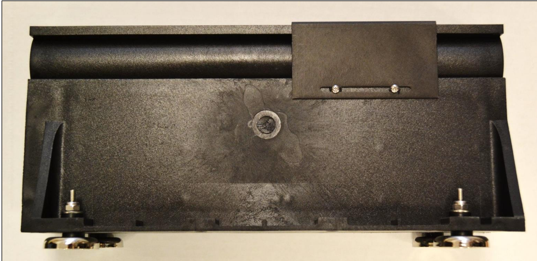
XL Magnetic Field Generator with CAM-External Photo Back Side View with shunt
