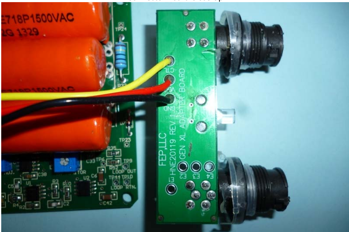
Connector Board Close Up
