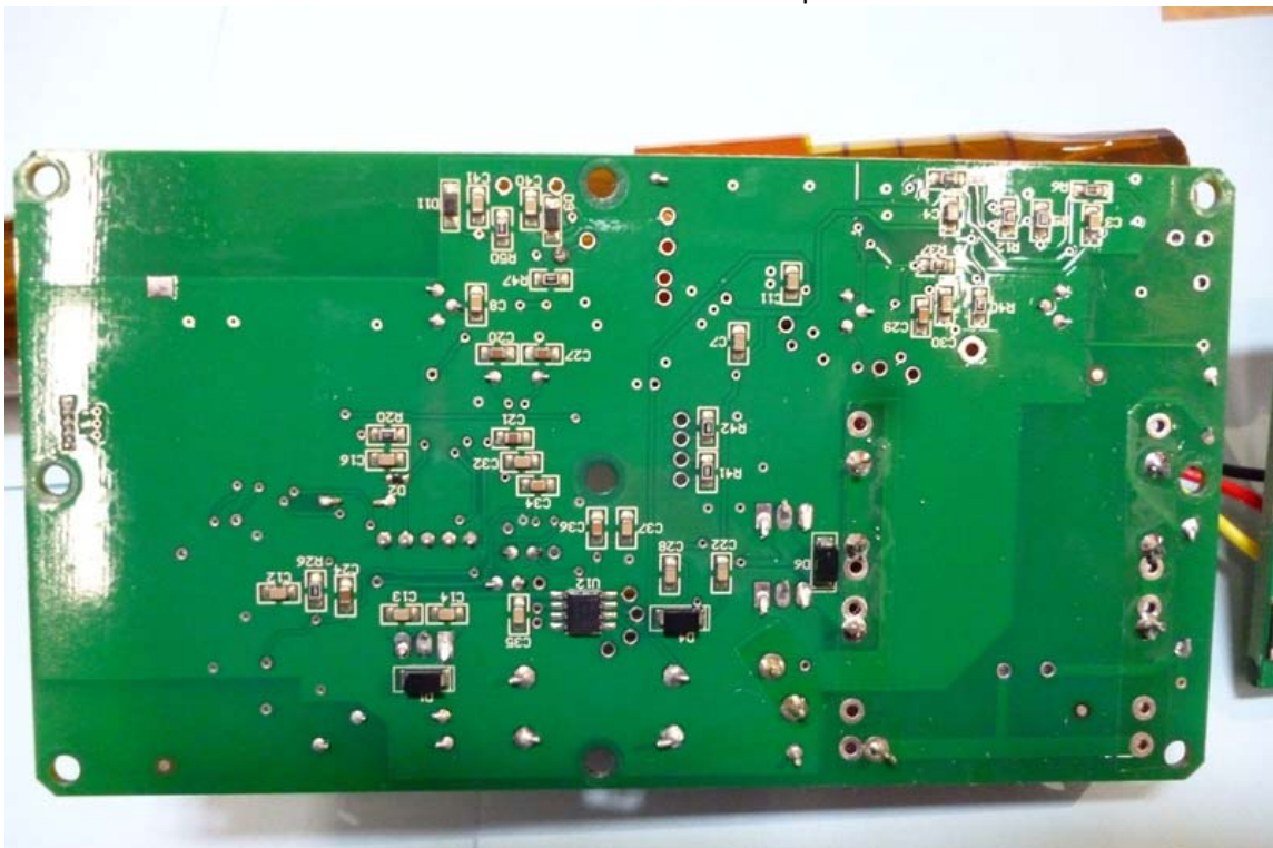
Board 2 – Bottom Close Up
