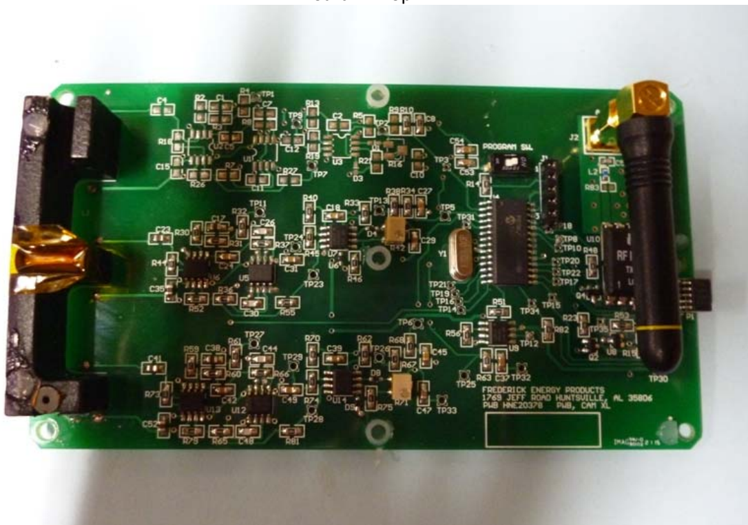
Board 1 - Top
