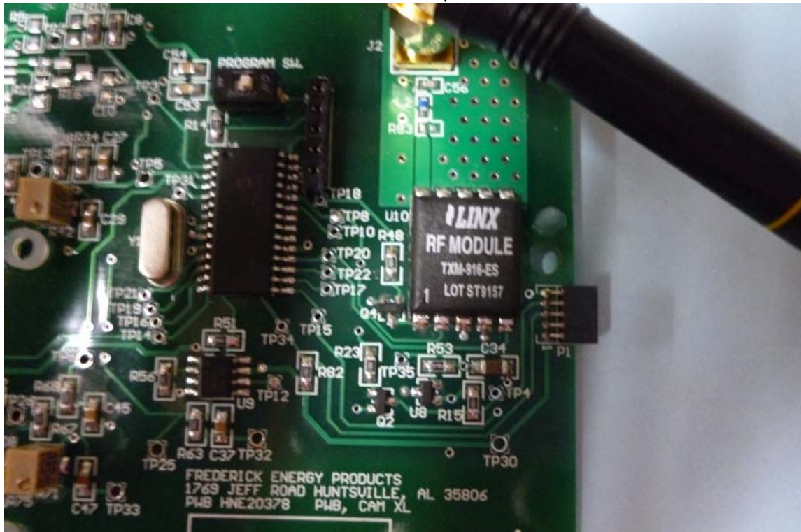
Board 1 – RF Circuit Close Up Antenna Turned
