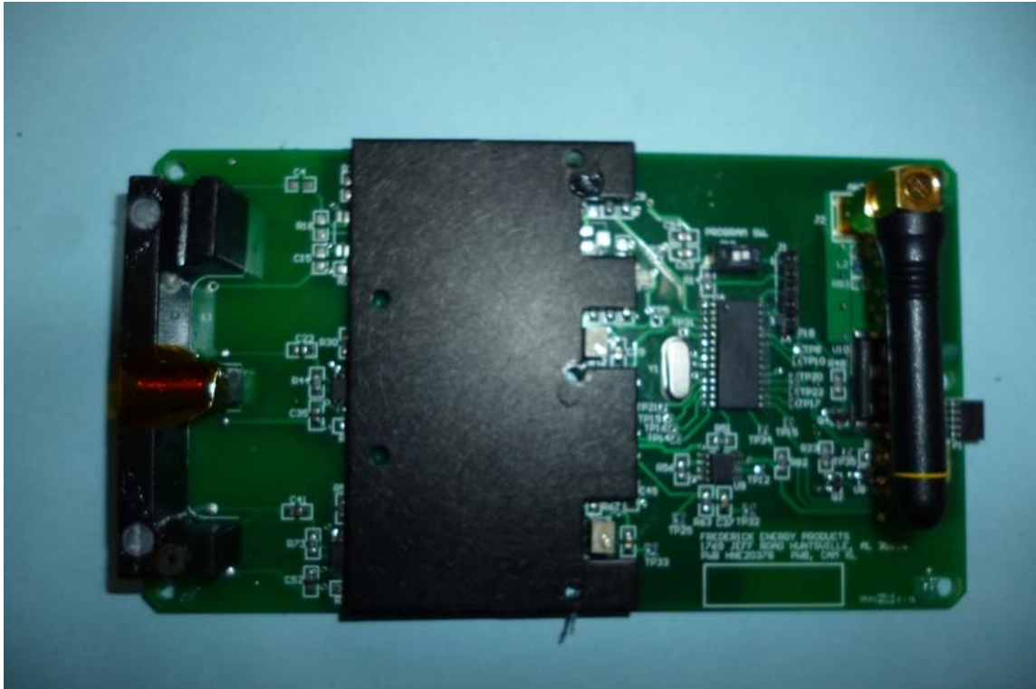
Board 1 with Cover
