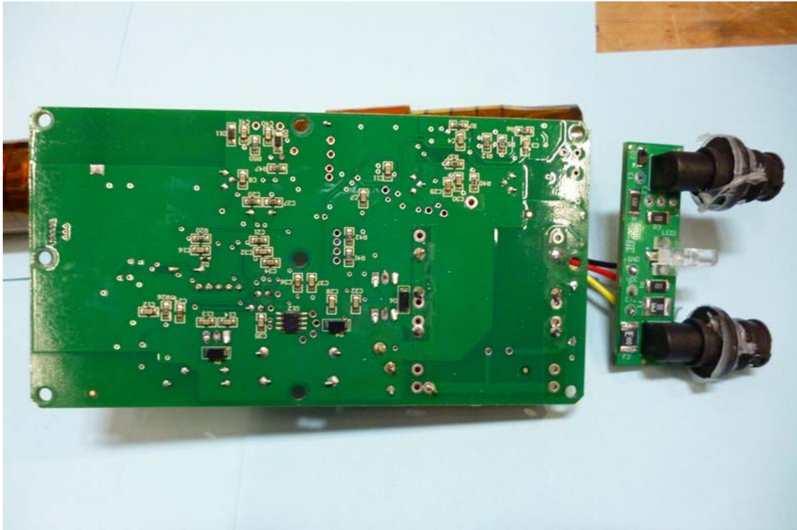
Board 2 - Bottom
