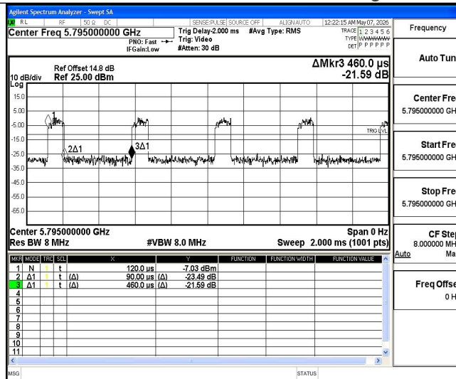
NTNV-11N40MIMO-Ant2-5795
