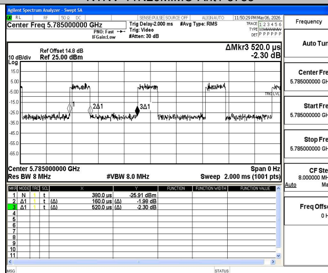
NTNV-11N20MIMO-Ant2-5785
