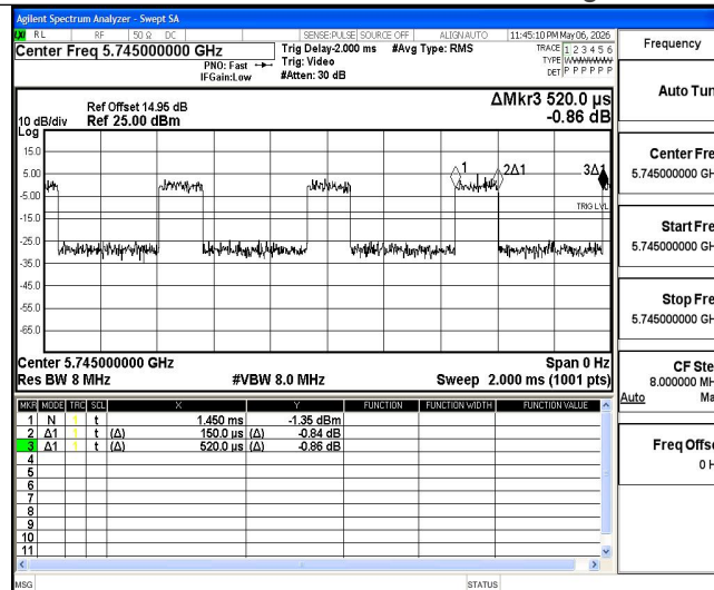
NTNV-11N20MIMO-Ant2-5745
