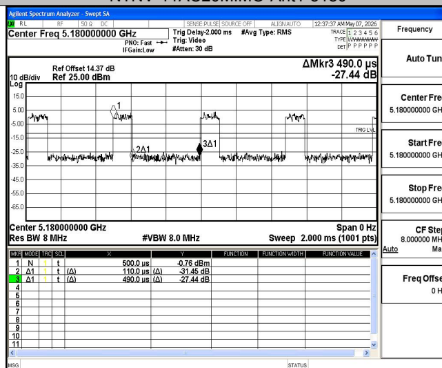
NTNV-11AC20MIMO-Ant2-5180
