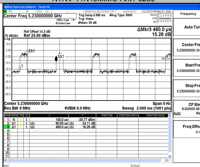
NTNV-11N40MIMO-Ant2-5230
