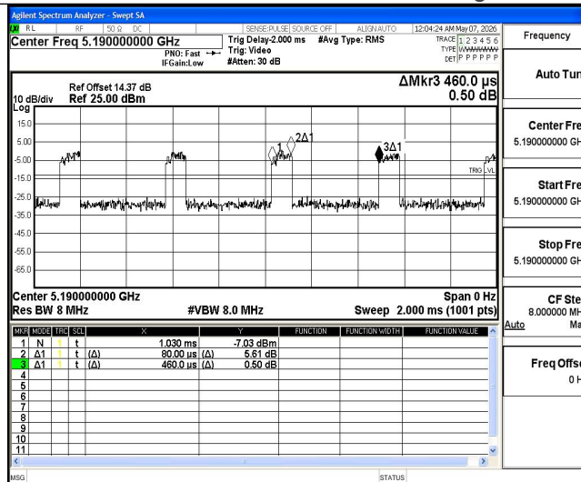
NTNV-11N40MIMO-Ant2-5190
