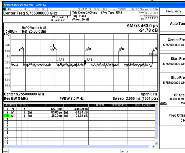
NTNV-11AC40MIMO-Ant2-5755
