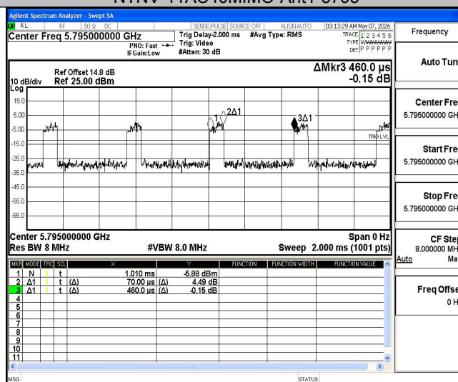
NTNV-11AC40MIMO-Ant2-5795
