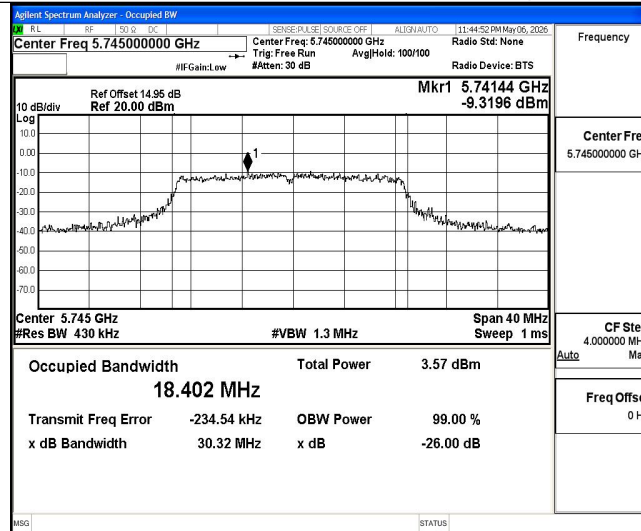
11N20MIMO-Ant2-5745
