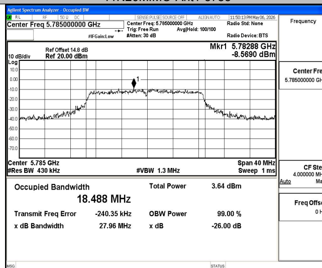
11N20MIMO-Ant2-5785
