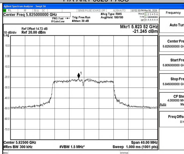
11A-Ant2-5825-PASS
