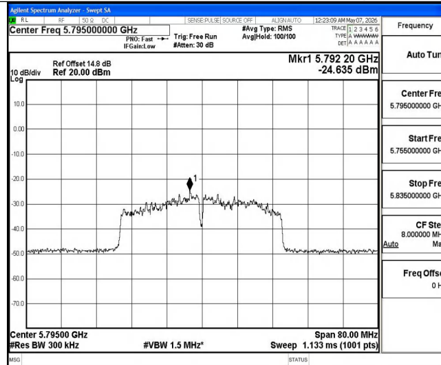
11N40MIMO-Ant2-5795-PASS
