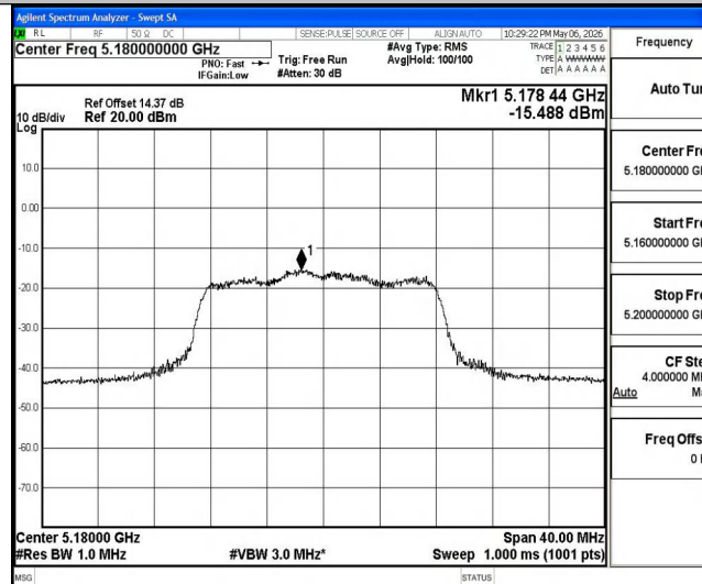
11A-Ant1-5180-PASS
