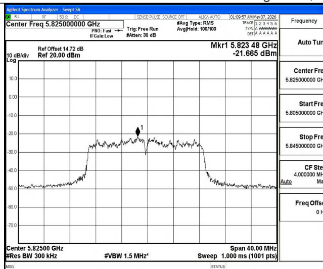
11AC20MIMO-Ant2-5825-PASS
