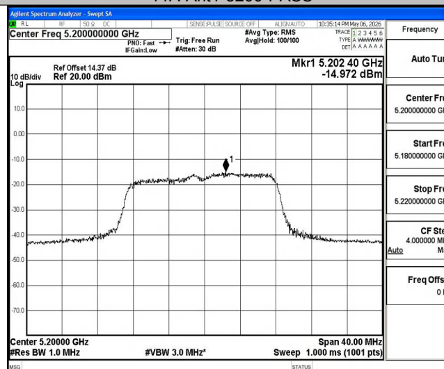
11A-Ant2-5200-PASS
