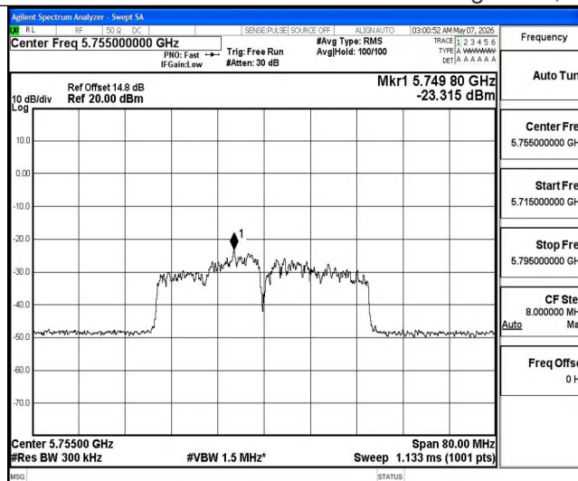
11AC40MIMO-Ant2-5755-PASS
