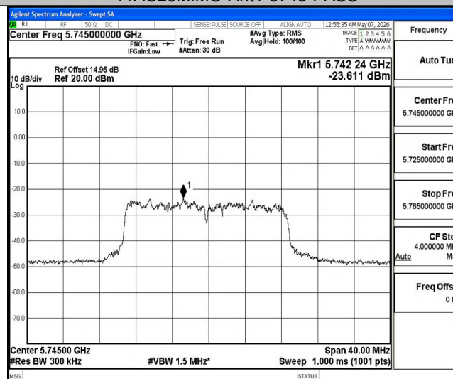
11AC20MIMO-Ant2-5745-PASS
