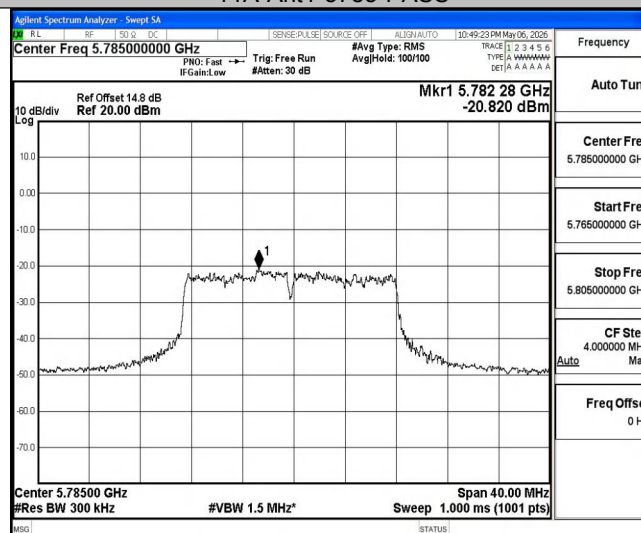
11A-Ant2-5785-PASS
