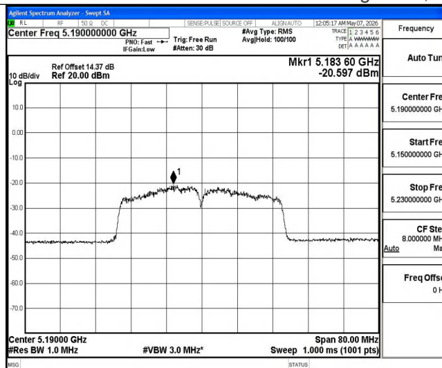
11N40MIMO-Ant2-5190-PASS
