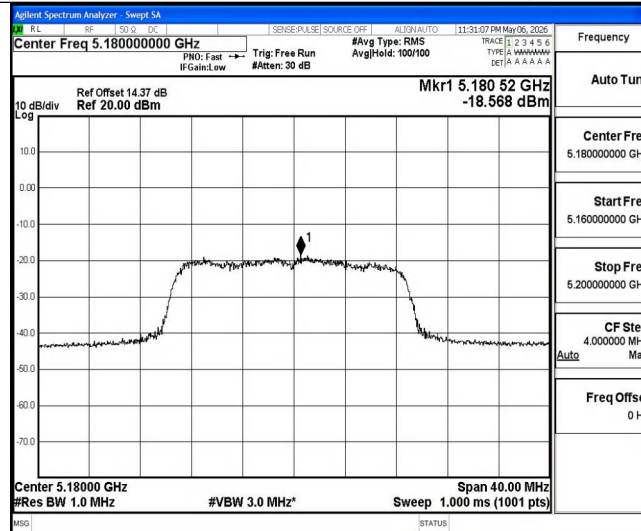
11N20MIMO-Ant2-5180-PASS
