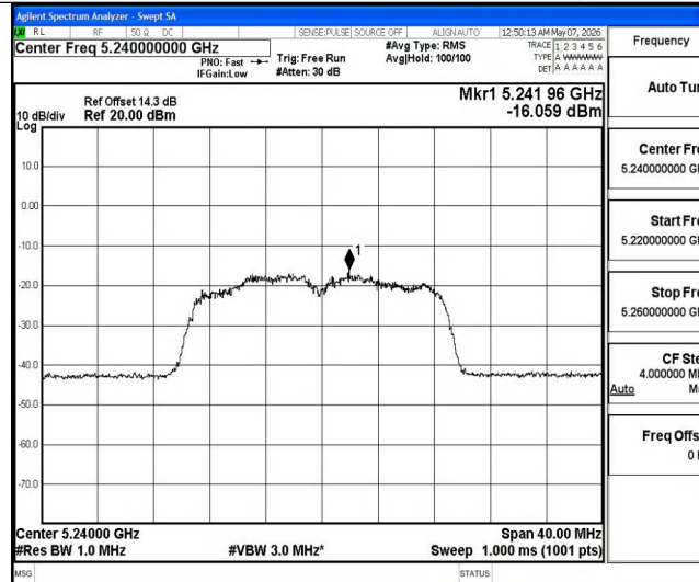
11AC20MIMO-Ant2-5240-PASS
