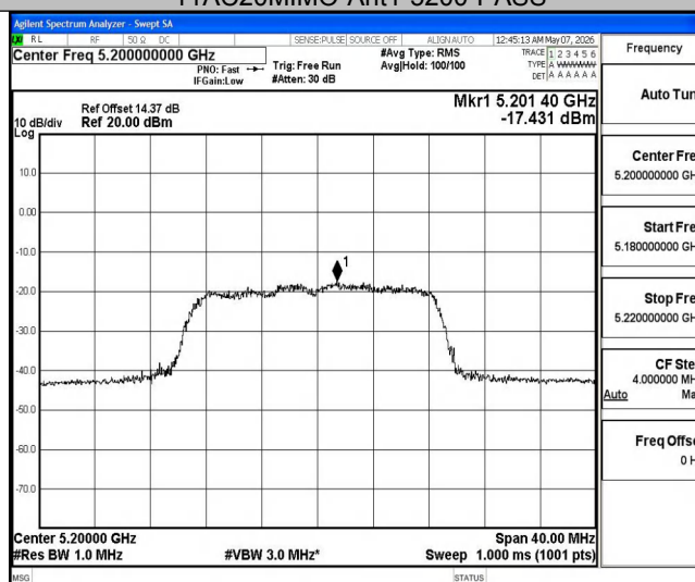
11AC20MIMO-Ant2-5200-PASS
