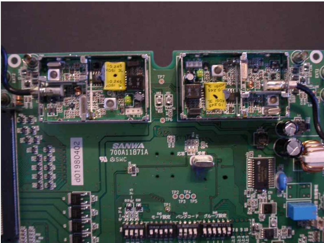
Internal Photo 2: Receiver Module shield Cover Removed
