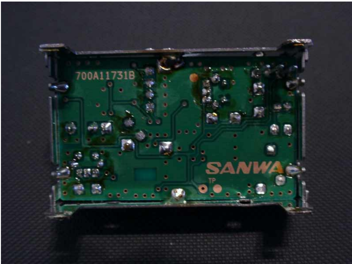
Internal Photo 3: Receiver Module bottom Side
