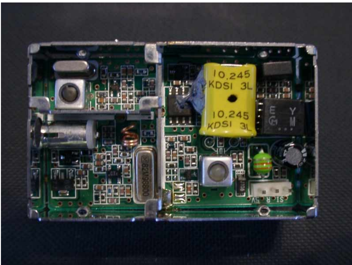
Internal Photo 4: Receiver Module Top Side
