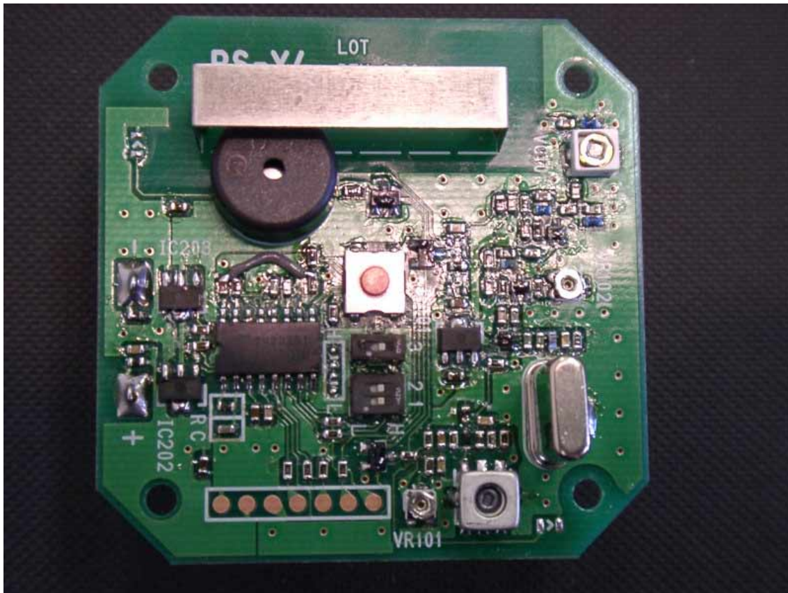
Internal Photo 1: Whole of Circuit Board Top Side
