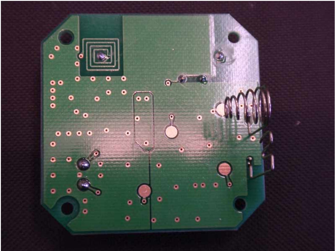
Internal Photo 3: Circuit Board Bottom Side
