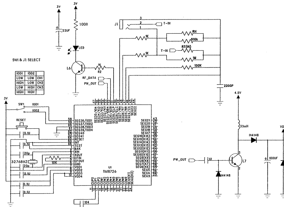
MCU CONTROL
