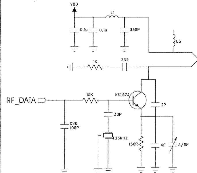
433.92MHZ TRANSMIT
