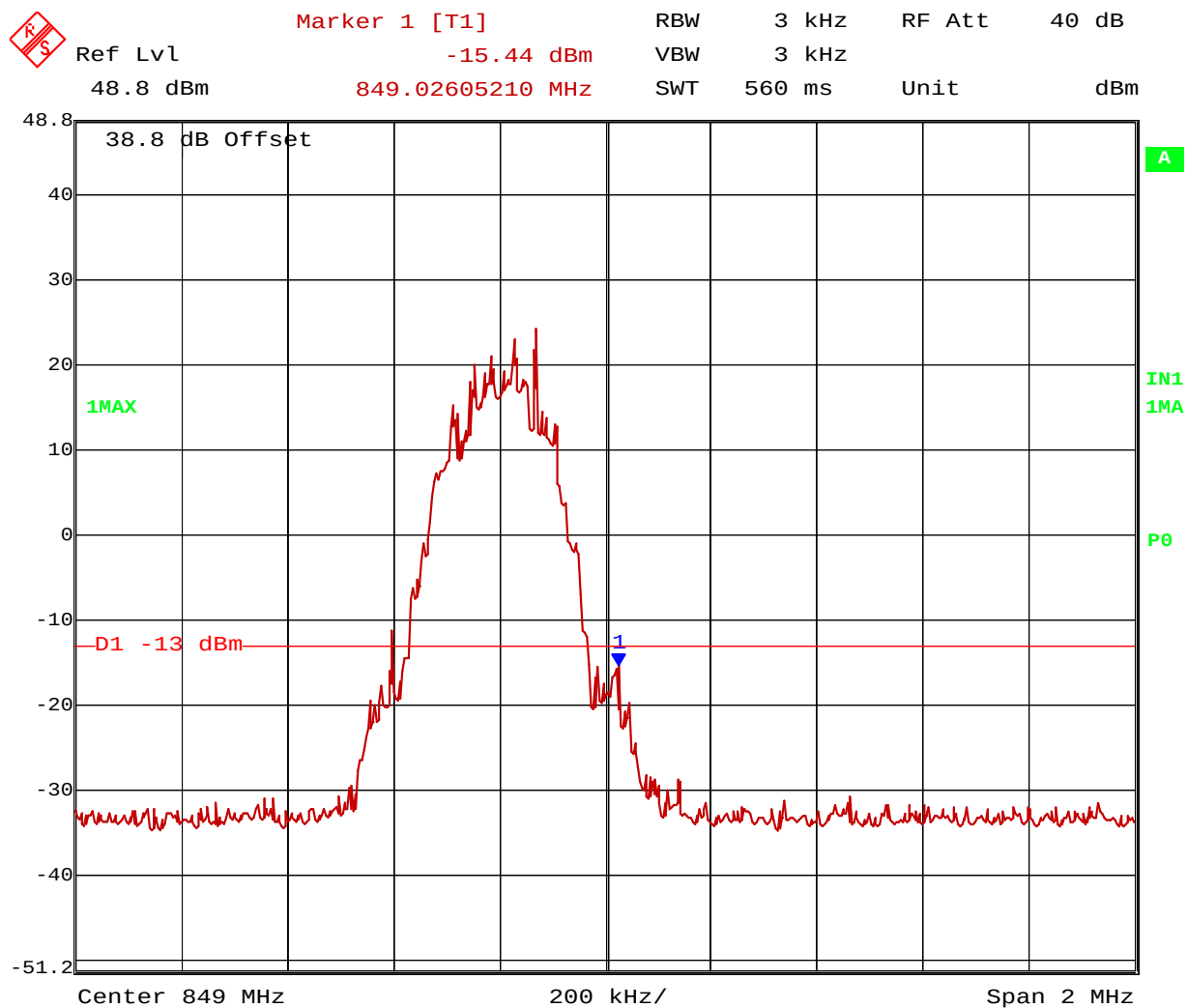
Figure 4 Upper bandedge, channel 251
