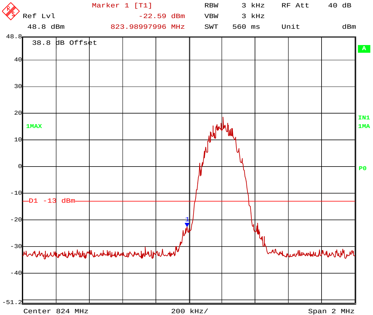
Figure 5 Lower bandedge, channel 128
