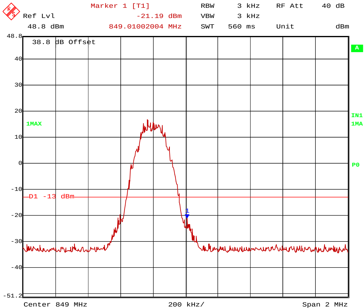
Figure 6 Upper bandedge, channel 251
