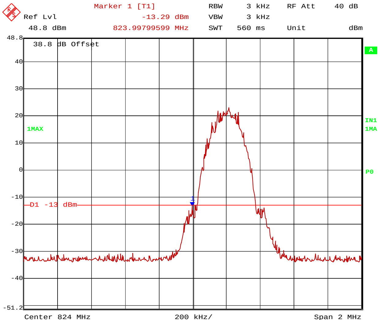
Figure 3 Lower bandedge, channel 128
