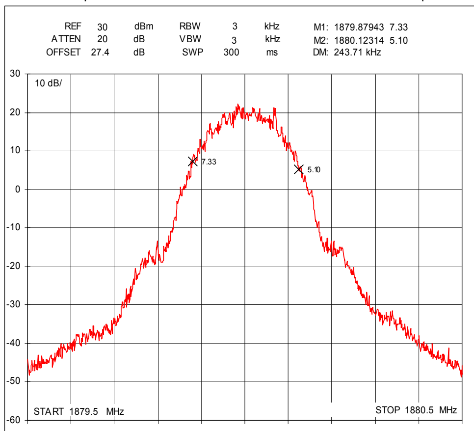
Spectrum analyzer plot channel 661, GMSK modulation
